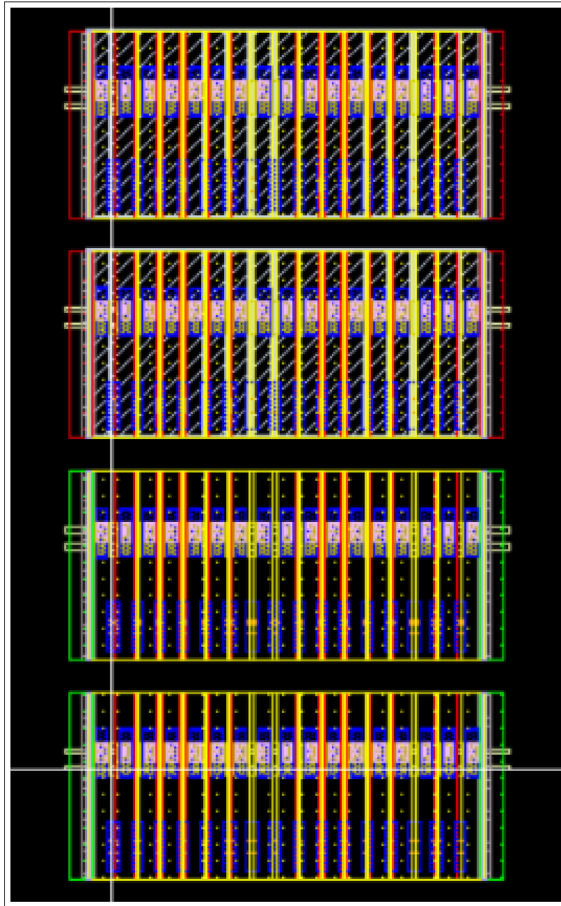
Figure 8.10: Native cellview of the Current Mirror successfully imported into Synopsys Custom Compiler via watchdog-triggered OpenAccess script injection.
