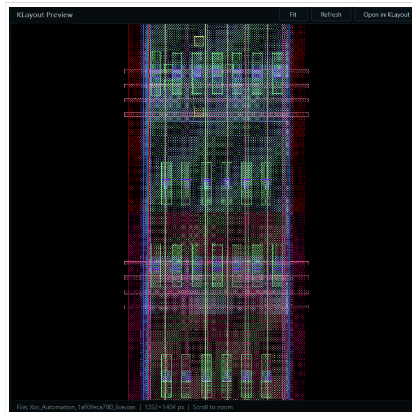
Figure 8.4: Final compacted and routed physical layout of the XOR gate cell in KLayout, showing snapped Metal 1/2 routing tracks and boundary clearances.
