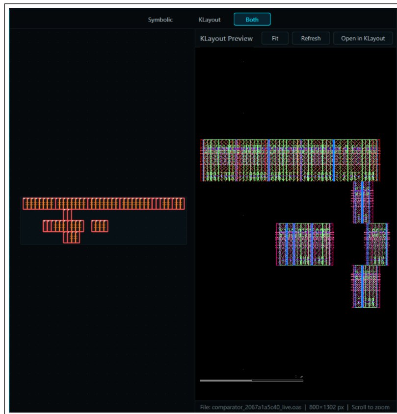
Figure 8.11: Initial uncompact symbolic placement of the Dynamic Analog Comparator cell, showing the latch and input pair layout template.
