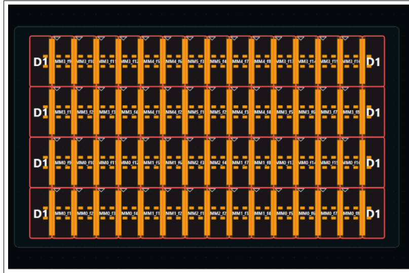
Figure 8.6: Symbolic placement of the Current Mirror with active diffusion sharing (abutment) and boundary guard ring outlines.
