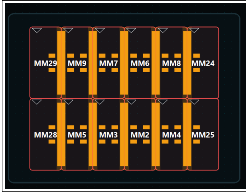
Figure 8.2: Symbolic placement of the XOR gate showing active region sharing (abutment) and initial row templates planned by the placement specialist.
