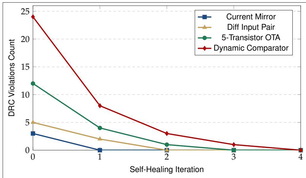
Figure 8.13: DRC Violation Self-Healing Convergence Curve across Agent Iterations.
