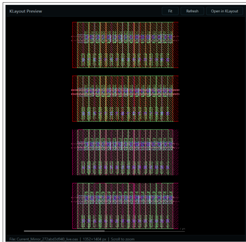
Figure 8.9: Final compacted GDSII cell layout of the current mirror in KLayout, showing shared diffusion regions and gate poly tracks.
