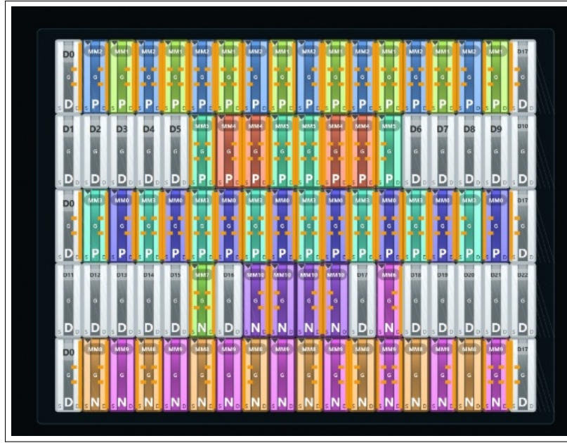
Figure 8.12: Final compacted and routed physical layout of the Dynamic Analog Comparator cell in KLayout, showing symmetrical device placement and guard rings.
