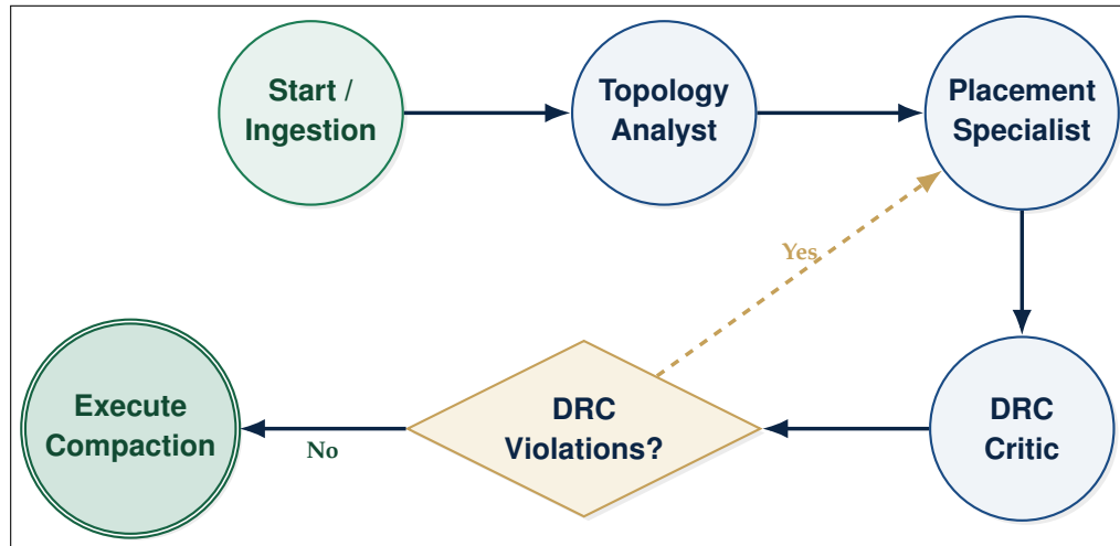
Figure 3.3: LangGraph Agent State Transition and Feedback Loop.
