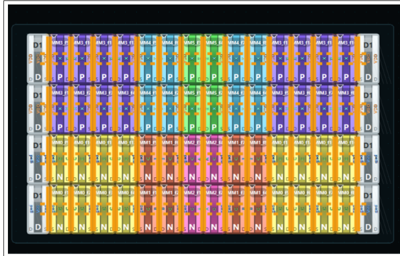
Figure 8.8: Color-coded transistor-level schematic detailing the matching patterns and common centroid routing plans for the current mirror.
