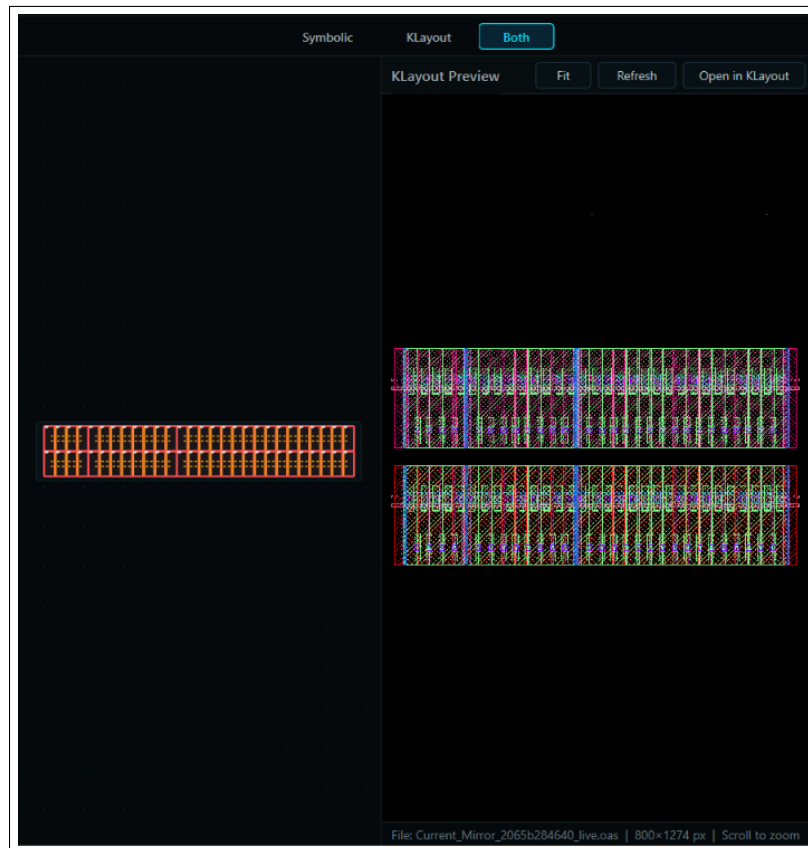
Figure 8.5: Initial uncompact placement of the 2-Transistor Current Mirror block, showing wide device separation and isolated active areas.
