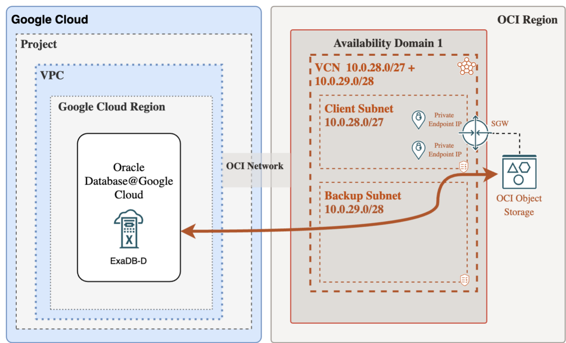
Automatic Backup to OCI Object Storage
