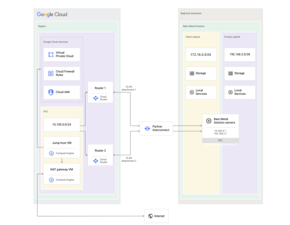
Figure 8: Current State Logical Architecture
