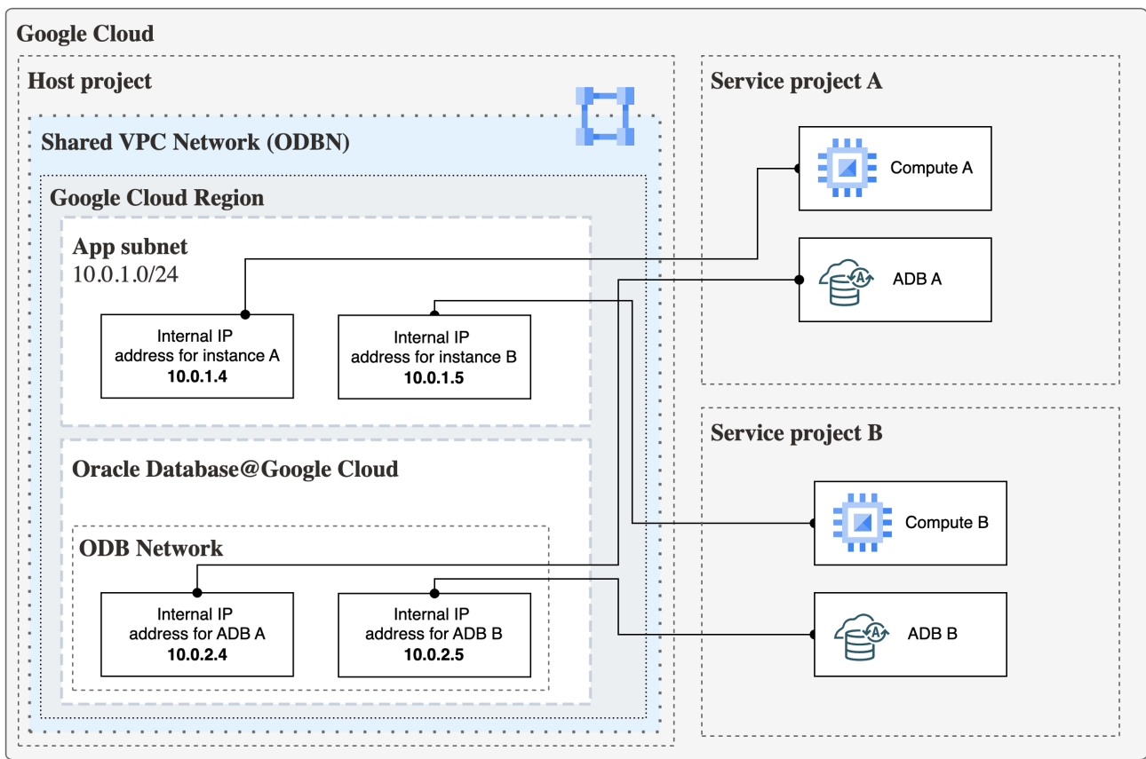
Figure 25: Oracle Database@Google Shared VPC architecture
