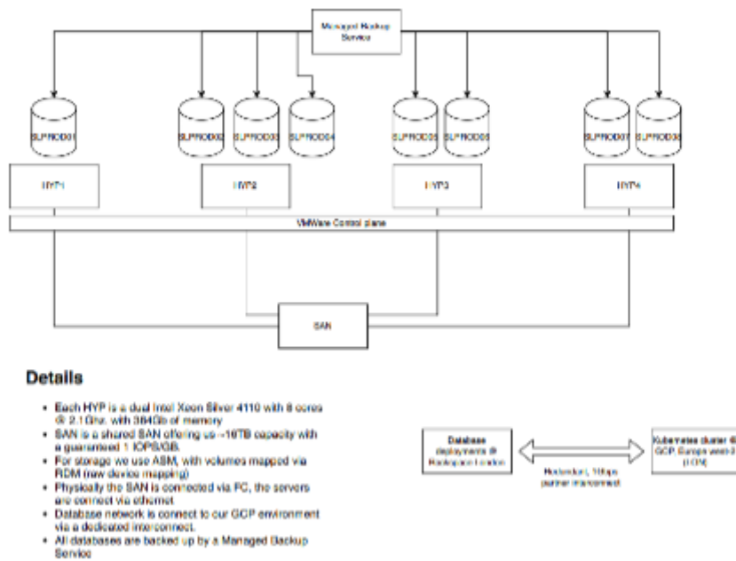
Figure 9: Current State Logical Architecture
