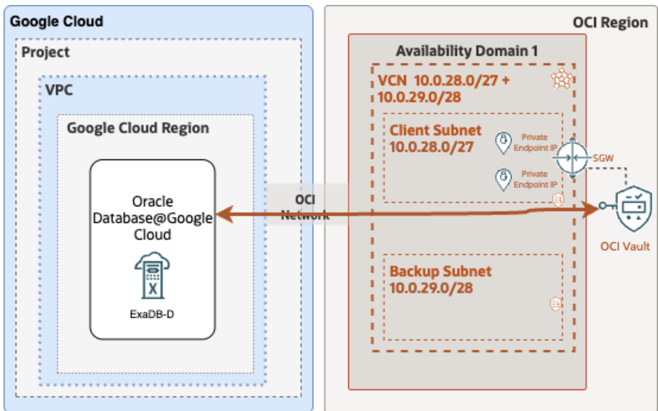
Figure 21: Oracle Database@Google Cloud with OCI Vault
