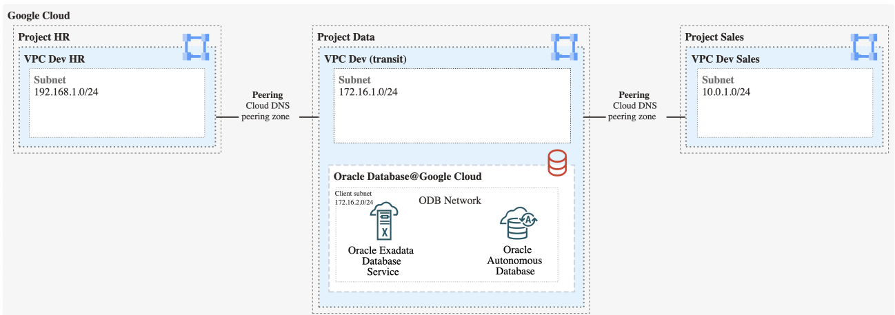
Figure 23: Oracle Database@Google Network Peering Topology
