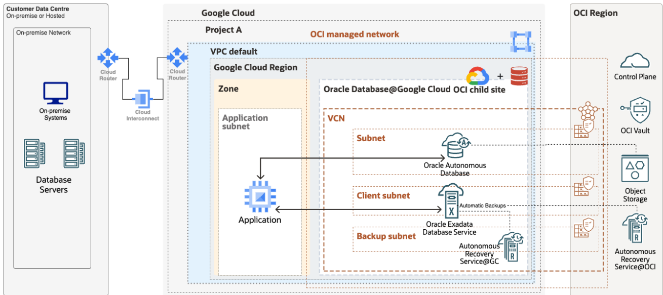
Figure 12: DB@Google High Level Deployment
