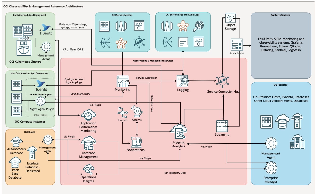
Figure 30: OCI Architecture
