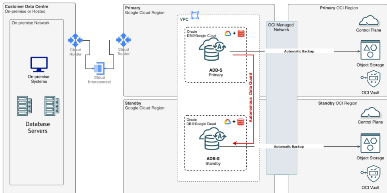
Figure 19: Oracle ADB-S@Google Multi-region Autonomous DataGuard
