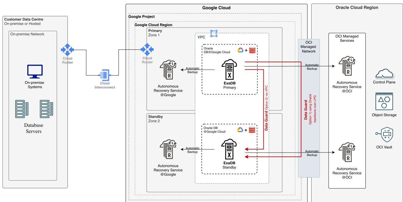
Figure 13: DB@Google MAA Gold Same Region
