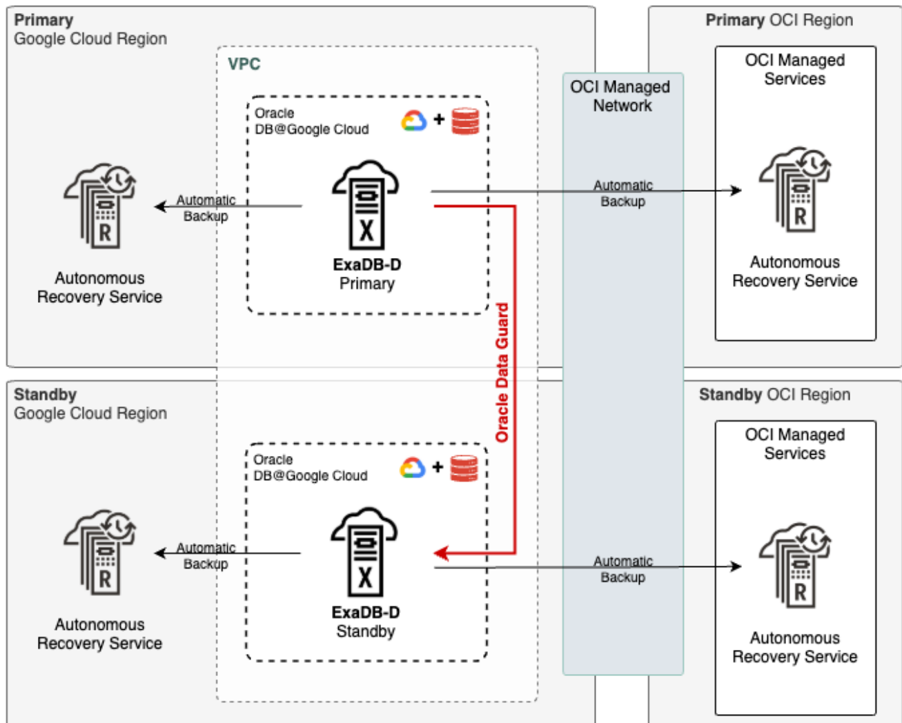
Figure 17: Oracle ExaDB-D@Google Cloud Multi-Region DR with Oracle Data Guard
