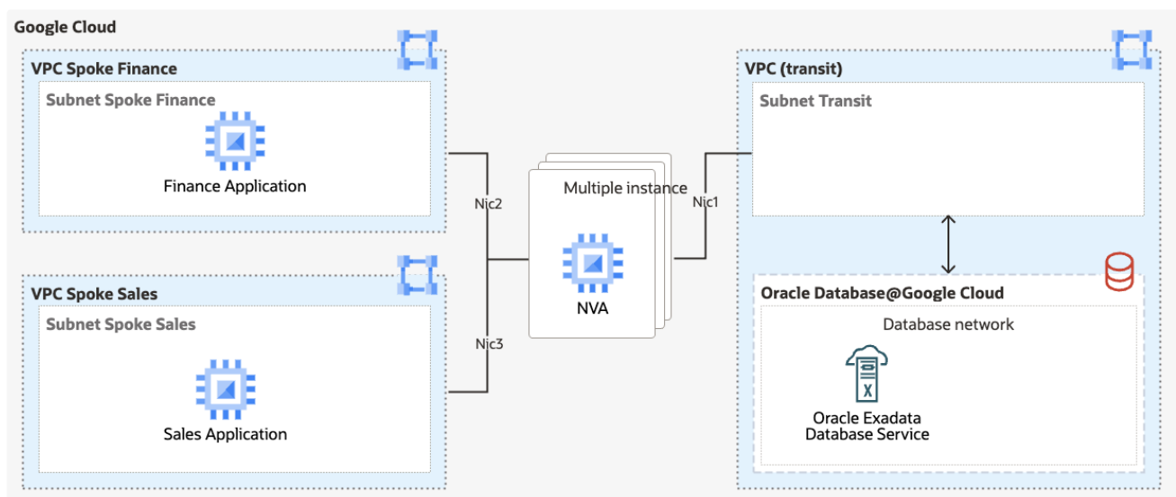
Figure 22: Oracle Database@Google Hub and Spoke Network Topology
