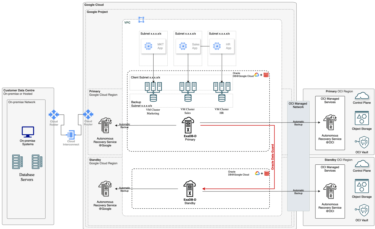
Figure 15: DB@Google Physical Across Regions
