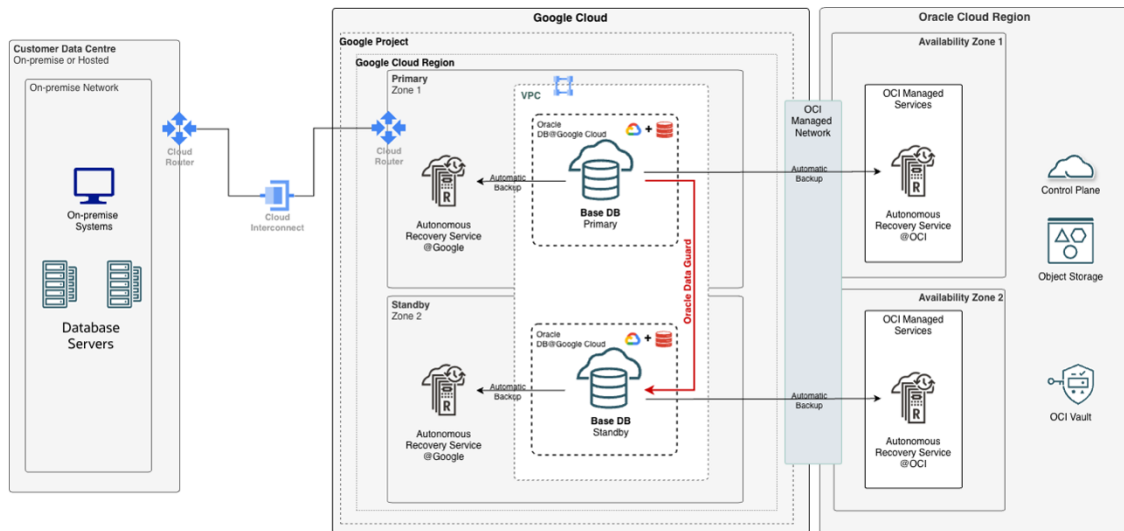
Figure 14: DB@Google MAA Gold Same Region
