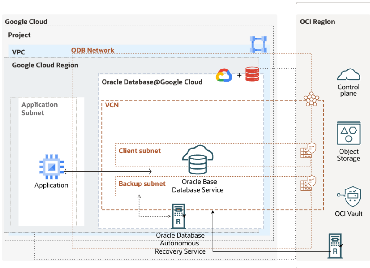
Figure 11: DB@Google Logical High Level
