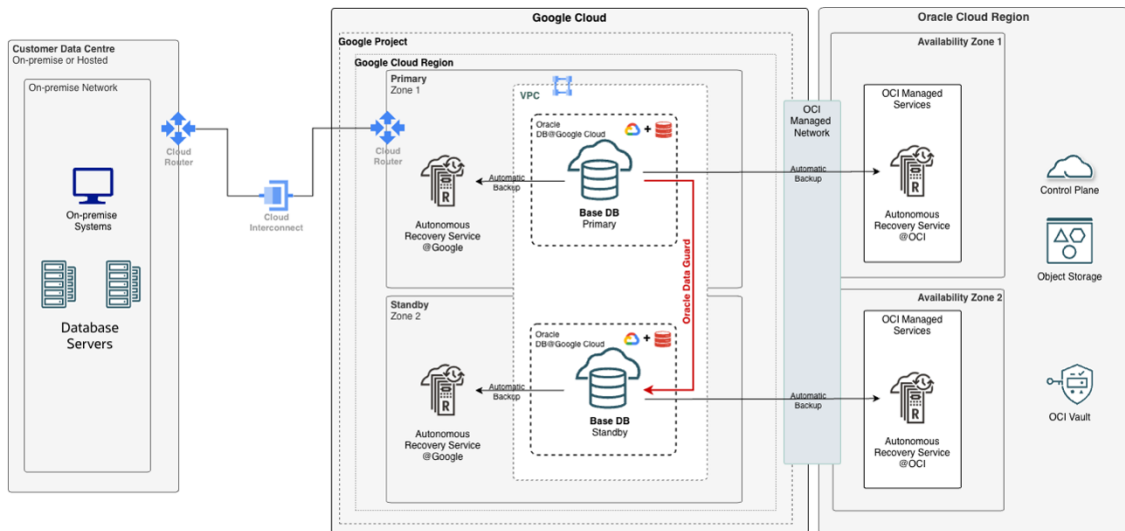
Figure 18: Oracle BaseDB@Google Cloud Multi-Region DR with Oracle Data Guard
