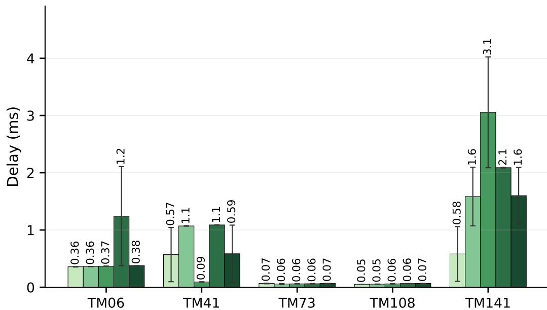
(c) Average Link Delay ↓
