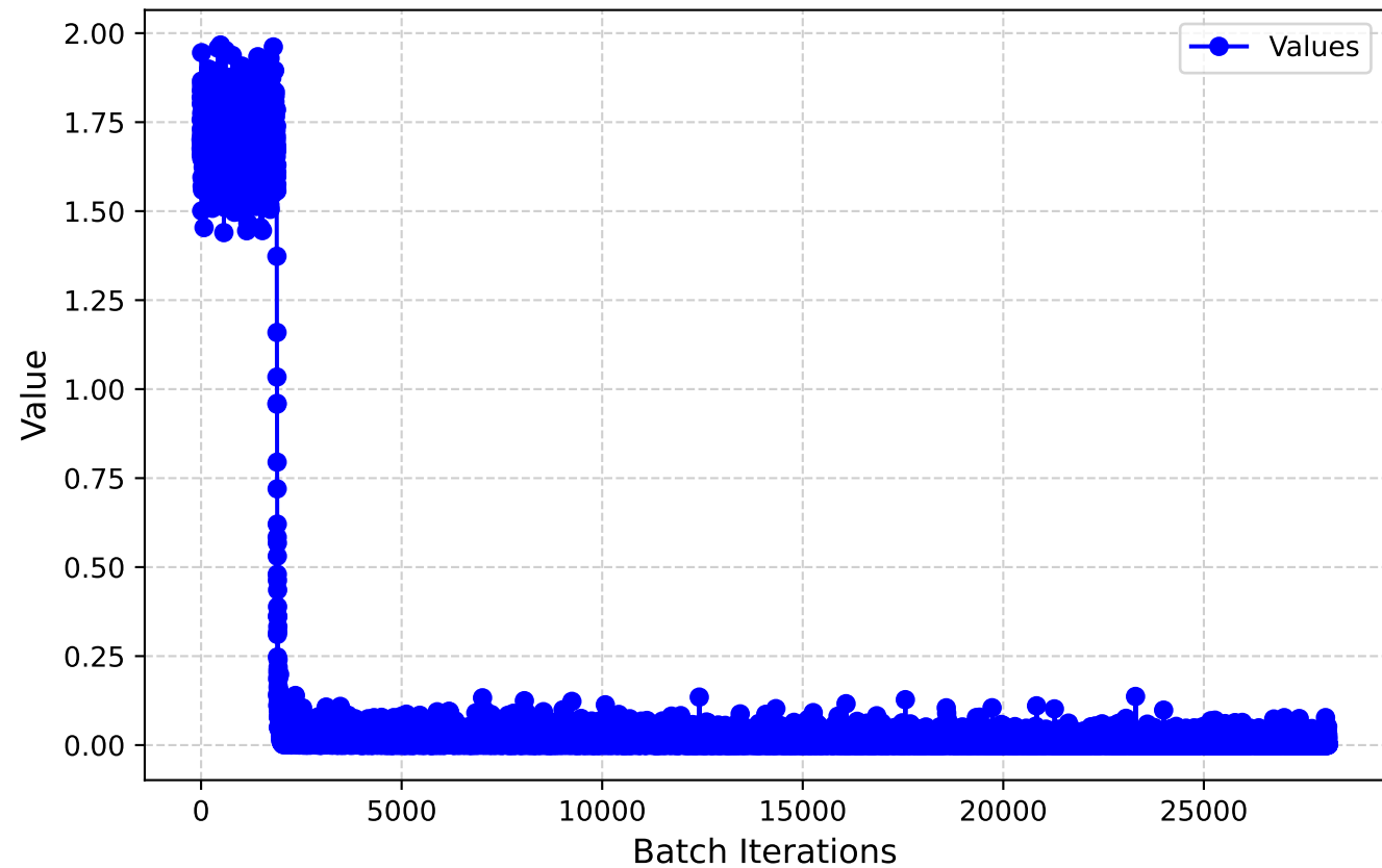
Prediction loss
