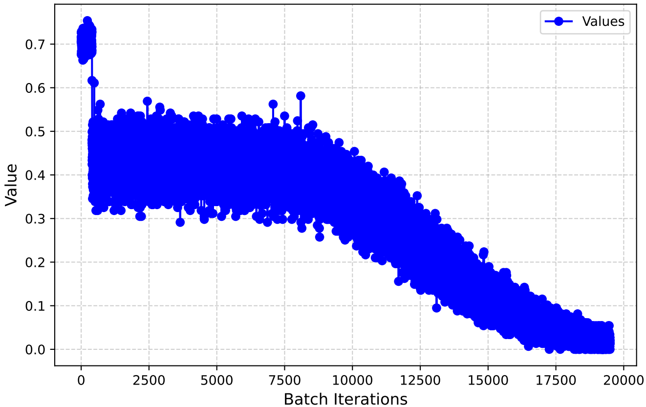
Prediction loss
