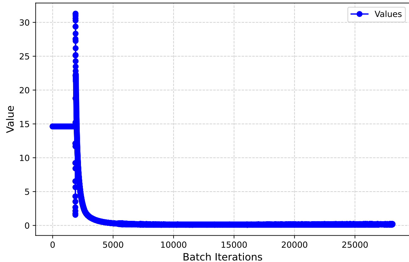
L2 loss
