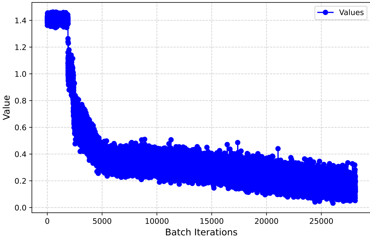
Prediction loss
