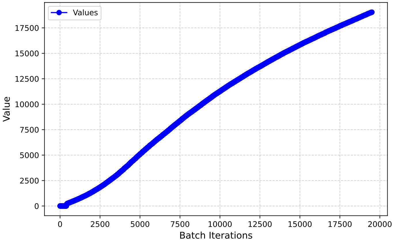
L1 loss
