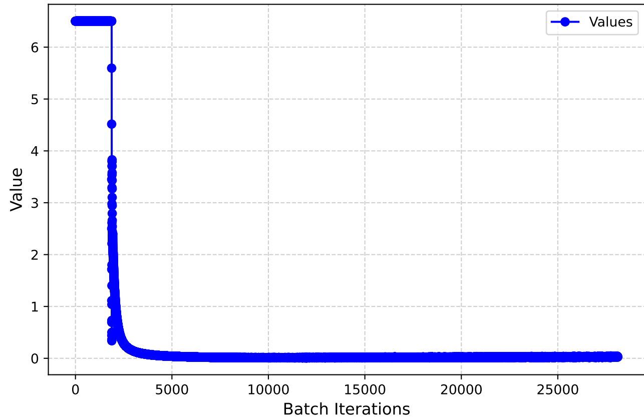
L2 loss
