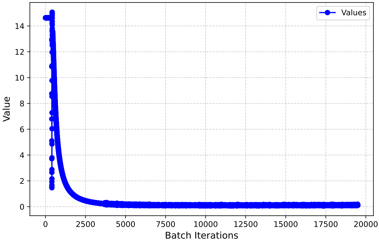
L2 loss
