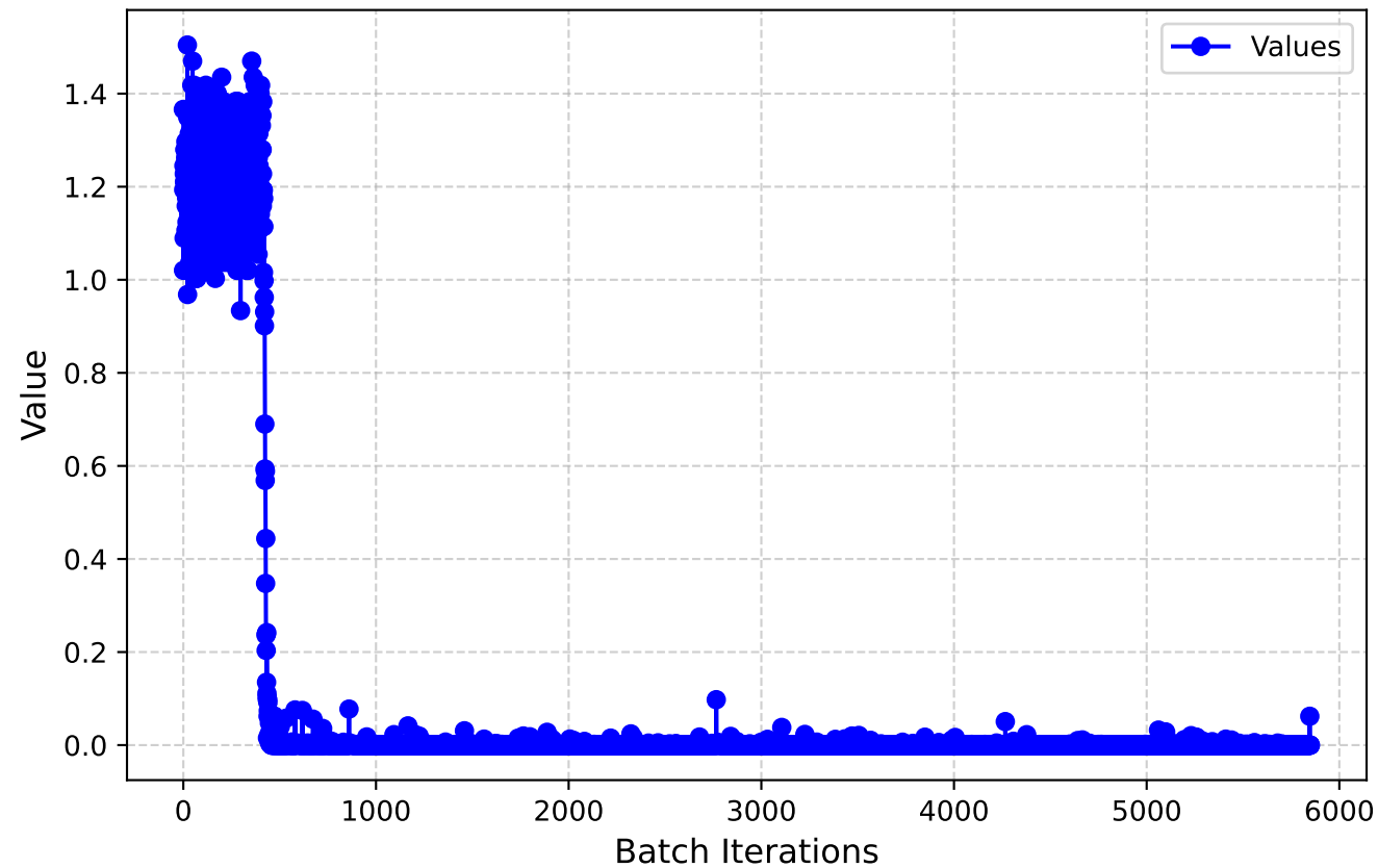
Prediction loss
