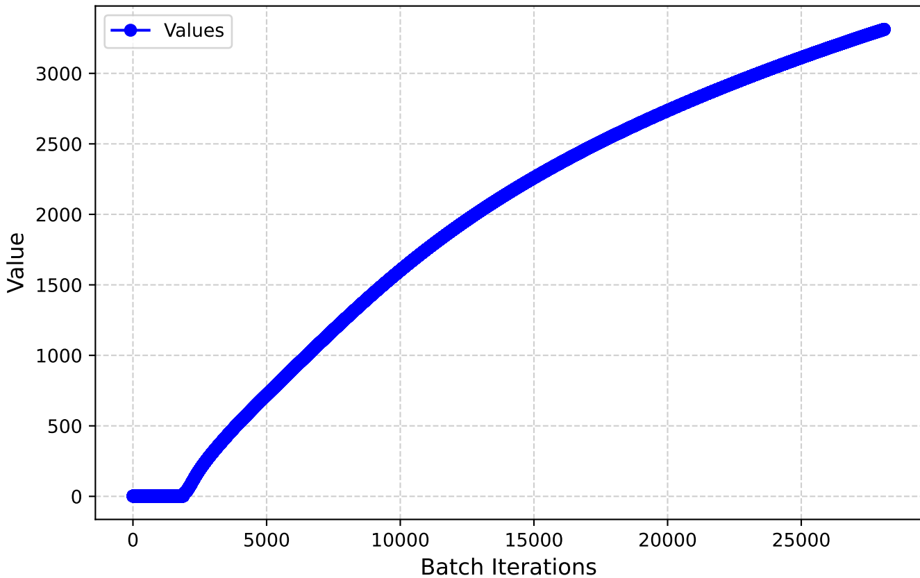
L1 loss
