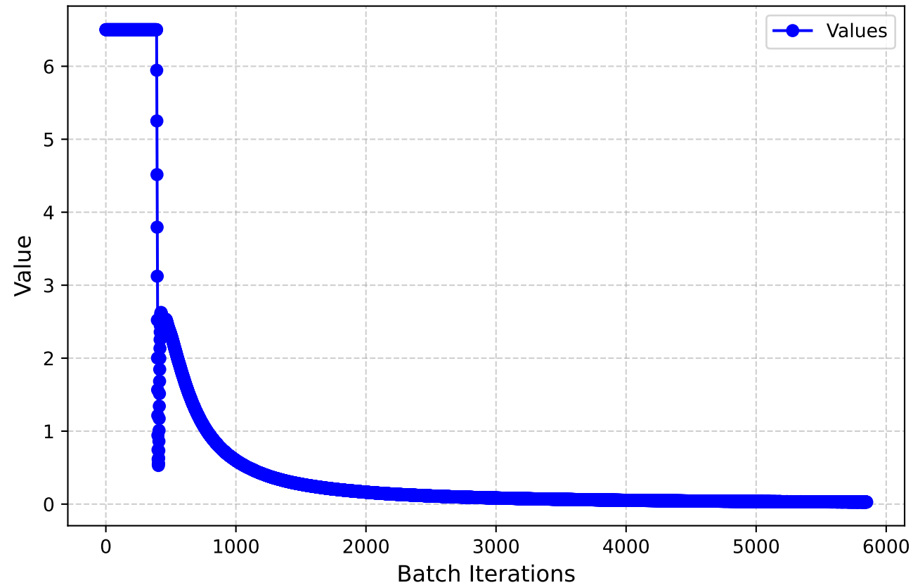
L2 loss
