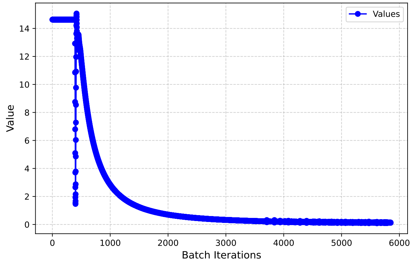
L2 loss
