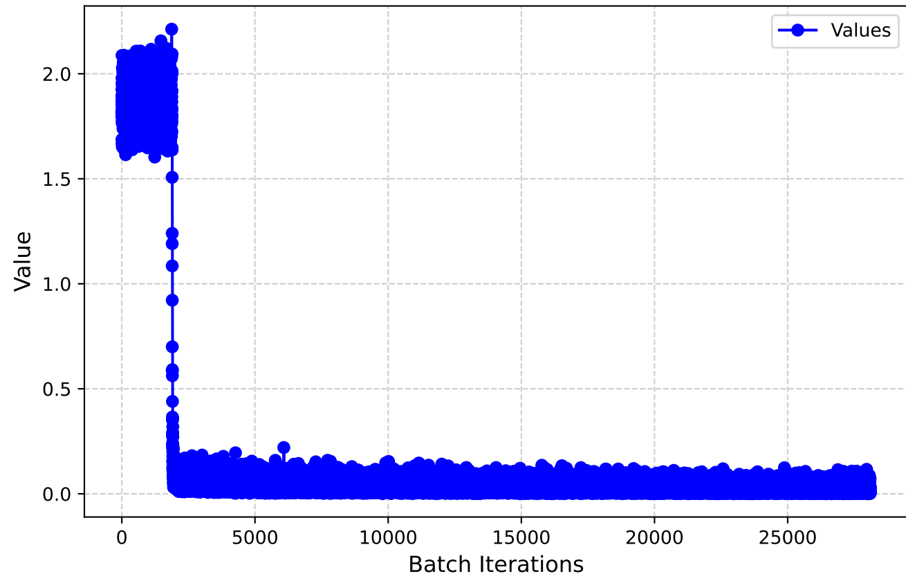
Prediction loss
