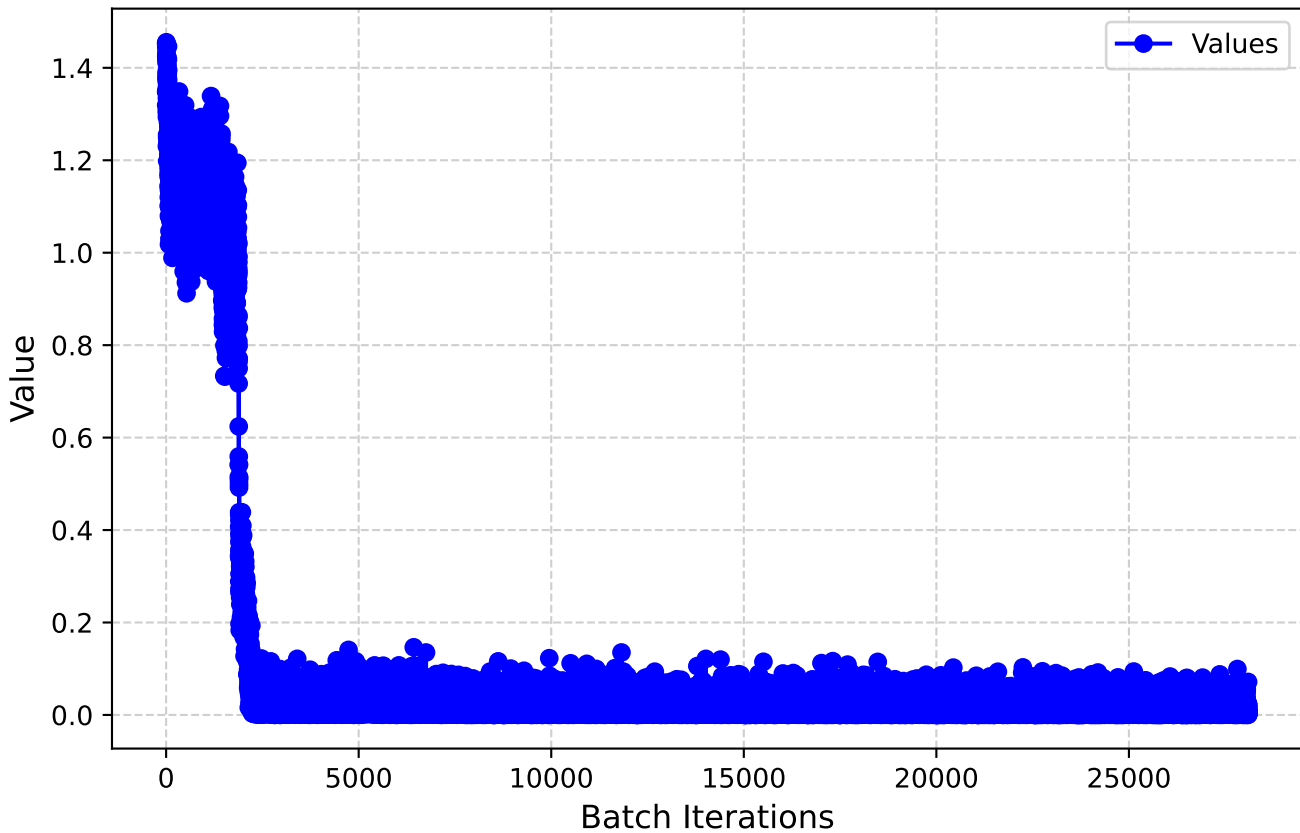
Prediction loss
