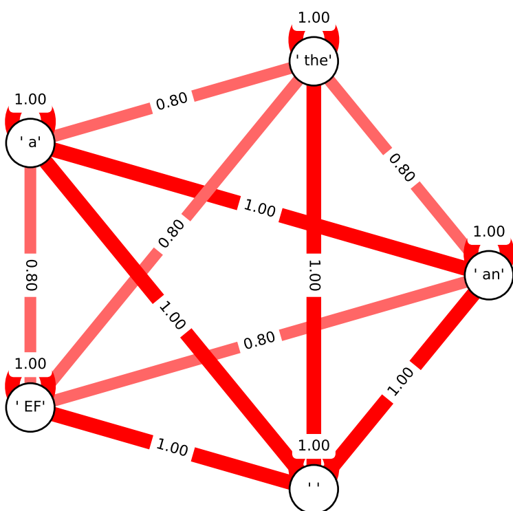
[Aleatoric] Non-Contradiction Graph
