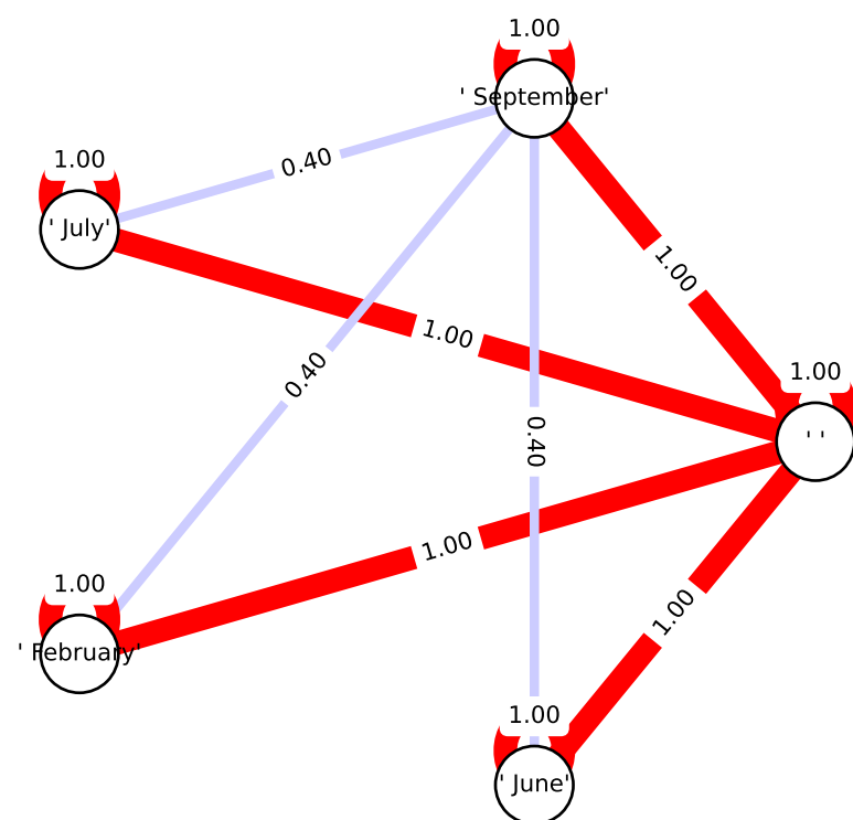
[Low uncertainty] Non-Contradiction Graph
