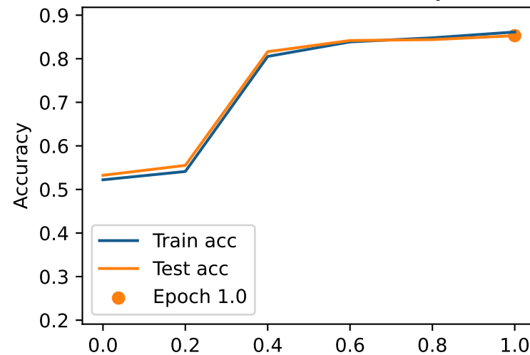
ETHICS/Mistral Accuracy
