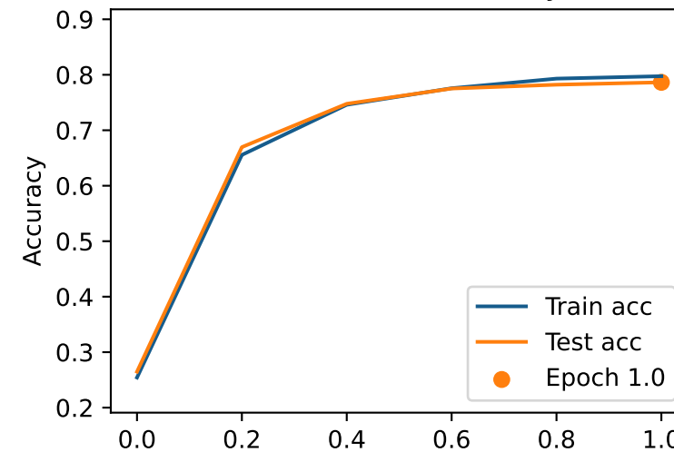
MMLU/Llama Accuracy
