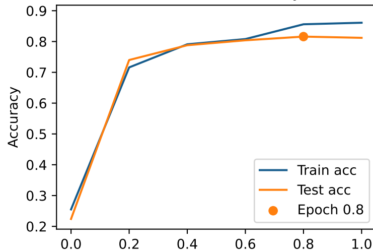
ARC/Mistral Accuracy
