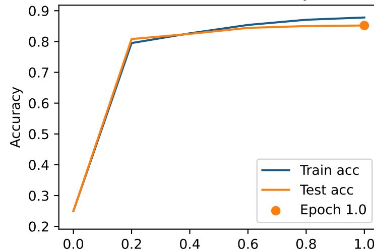
MMLU/Mistral Accuracy
