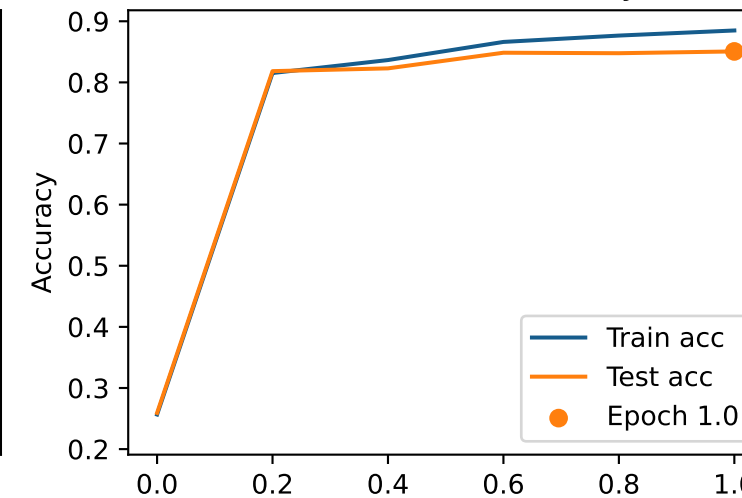
MMLU/Gemma Accuracy
