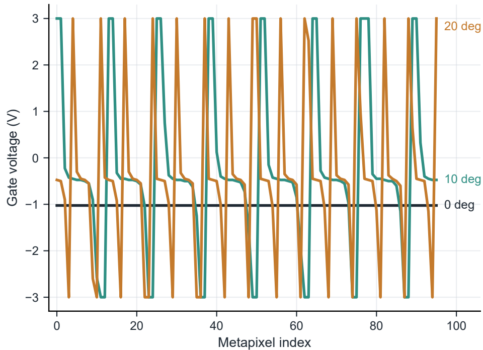
Inverse-designed voltage maps
