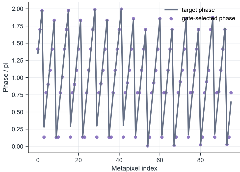
Phase quantization for 20 deg steering
