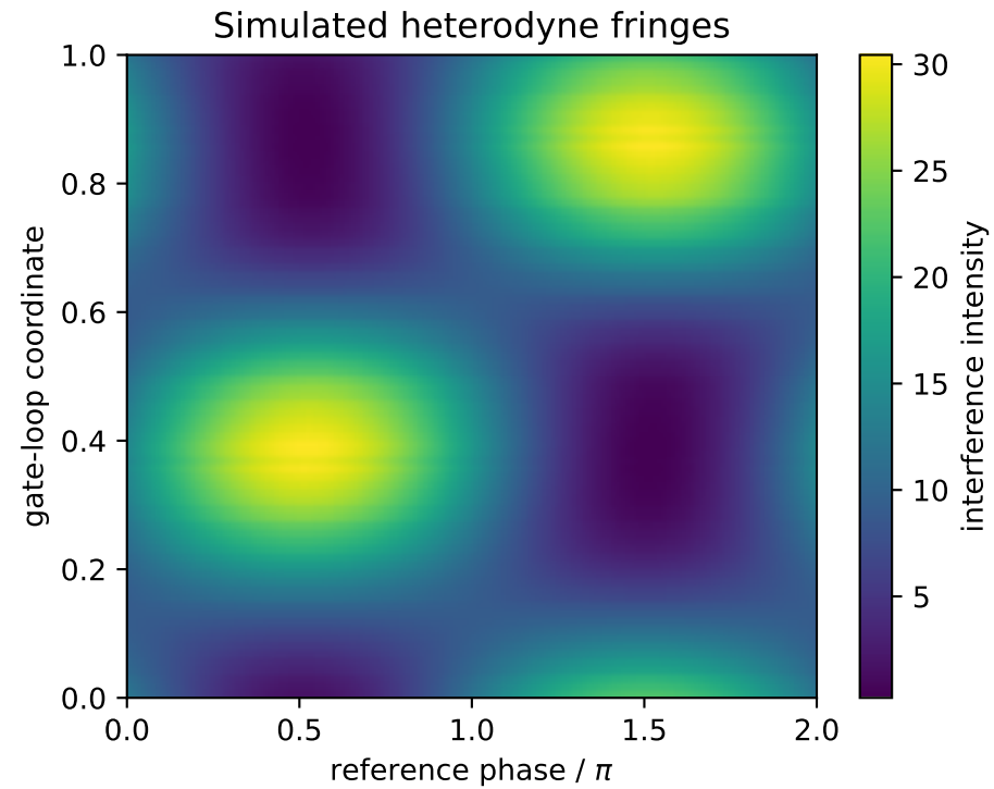
Figure 5. Heterodyne SHG observable
