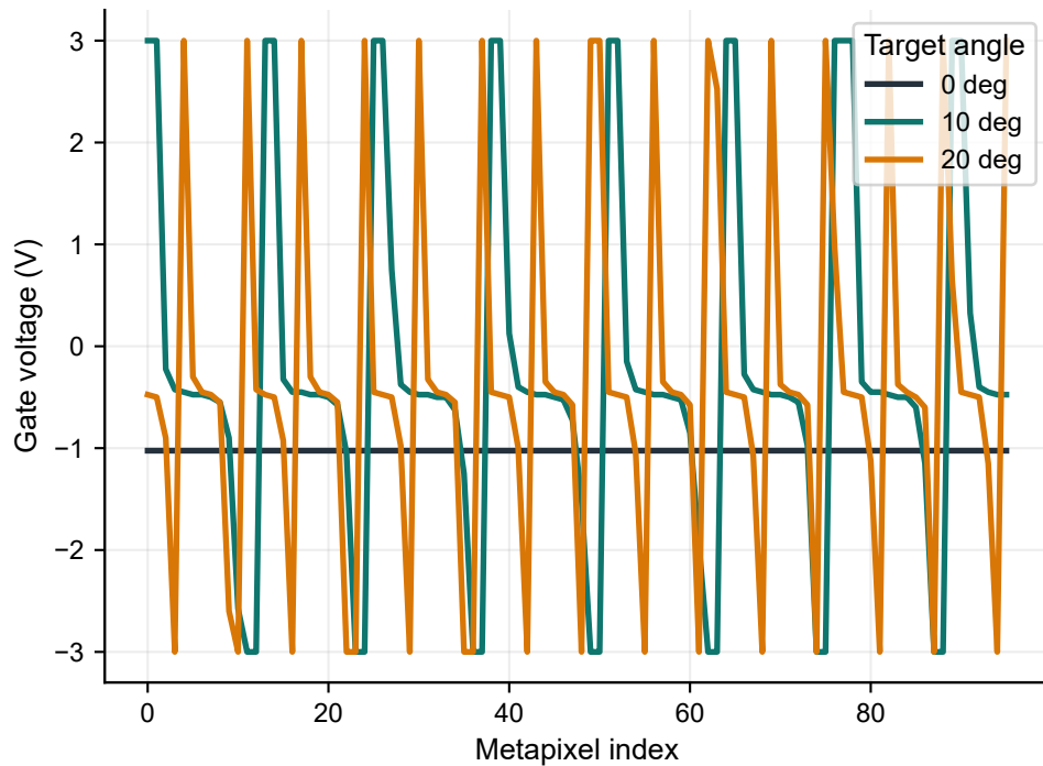
Inverse-designed gate profile
