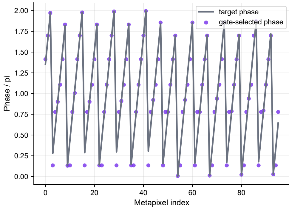
Phase matching for 20 deg steering
