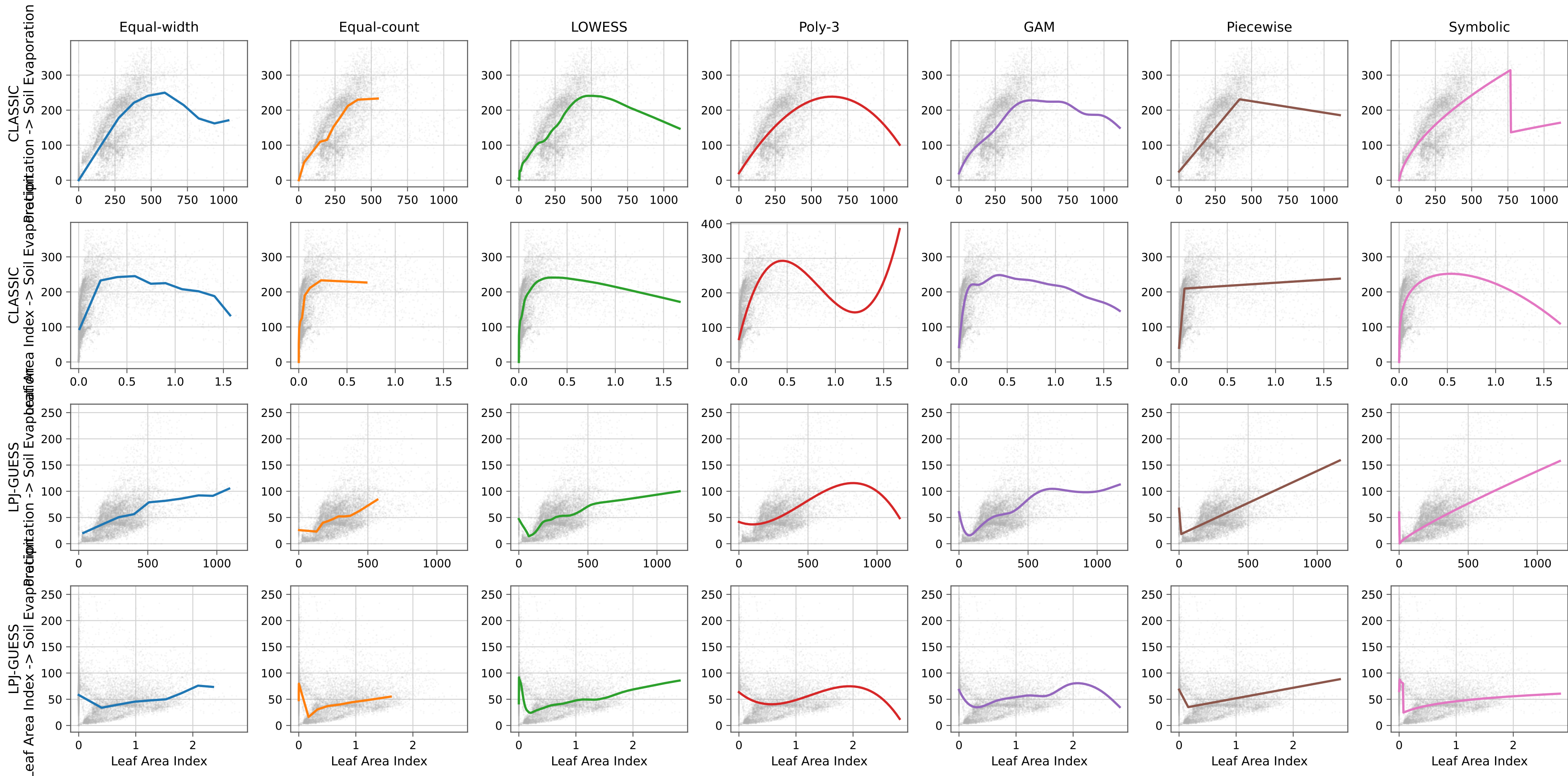
CD - Cold-Dry: one fitting method per panel for Soil Evaporation
