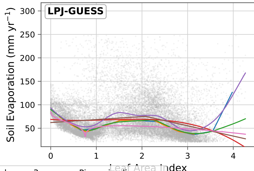
Leaf Area Index -> Soil Evaporation
