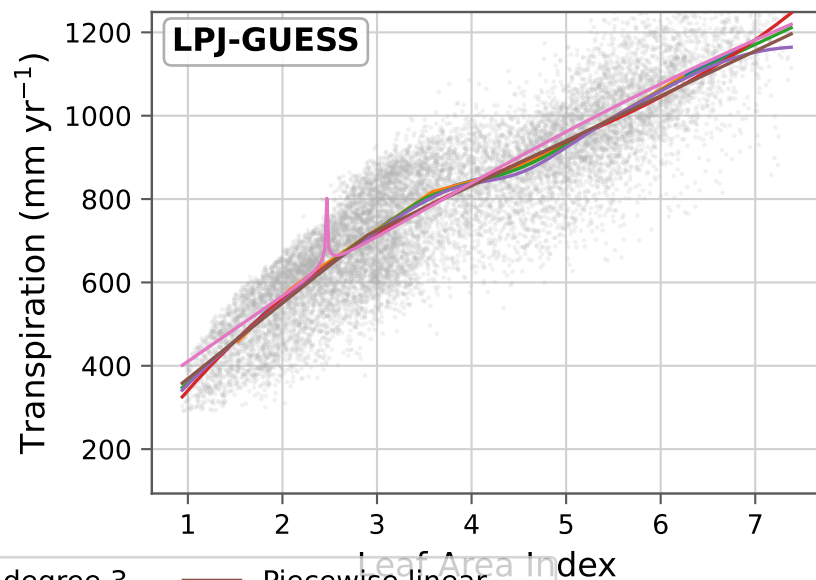
Leaf Area Index -> Transpiration
