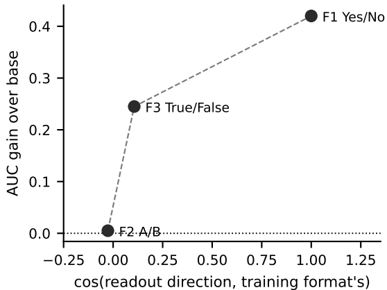
(a) transfer tracks readout direction
