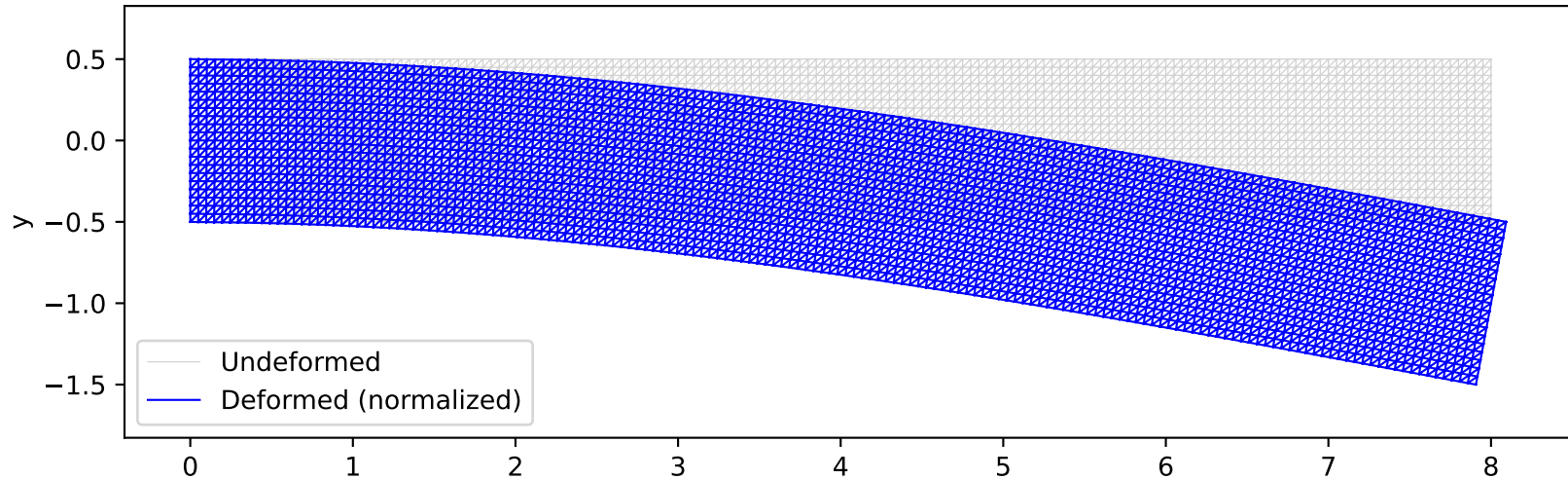
Cantilever Beam: Deformed Configuration
