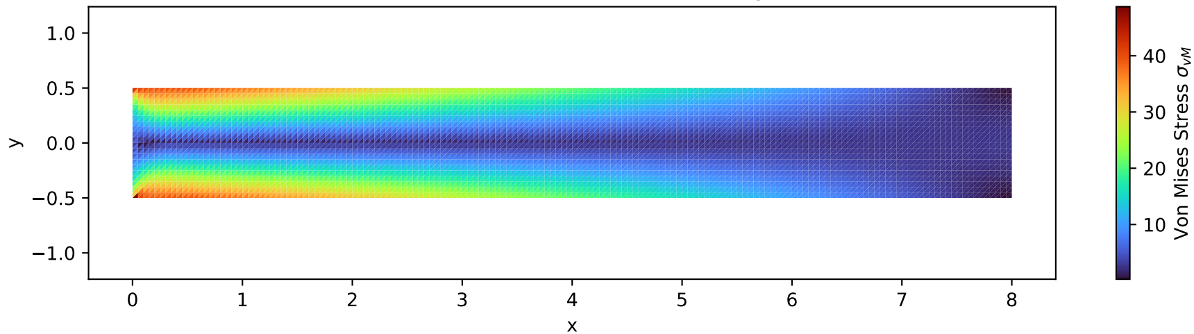
Von Mises Stress Field (Undeformed Configuration)
