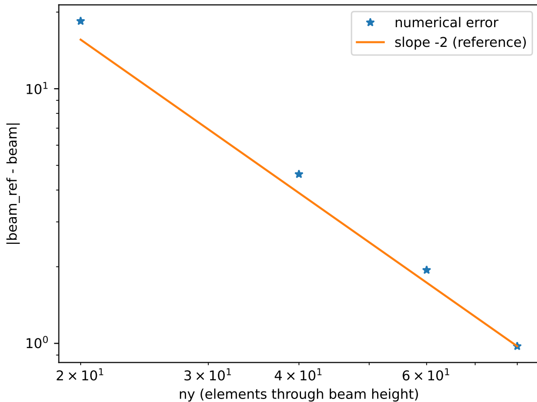
Error behaviour (observed order 2.11)
