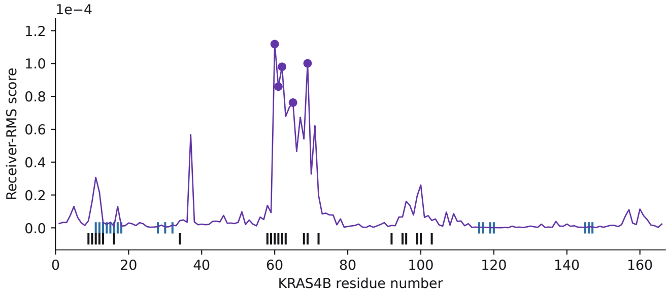
The two-mode shortlist clusters in switch II
