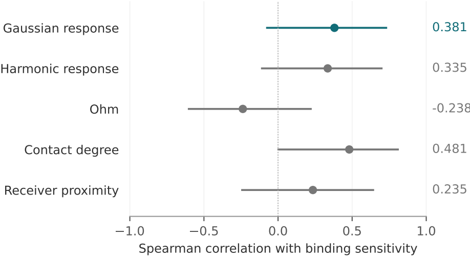
Observed association and 95% intervals
