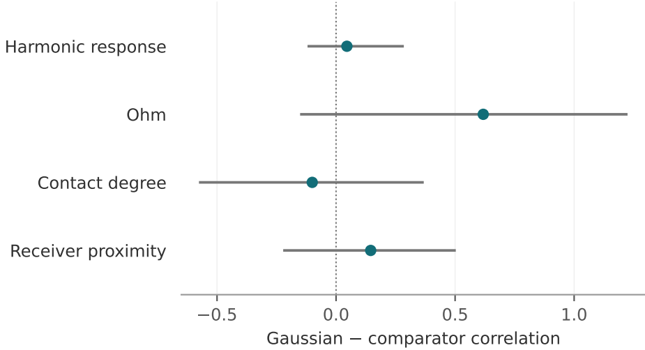
Paired differences and 98.75% intervals
