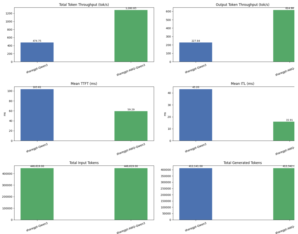
Qwen3-14B and Quantitized model vLLM Serving Performance Comparison on ShareGPT dataset
