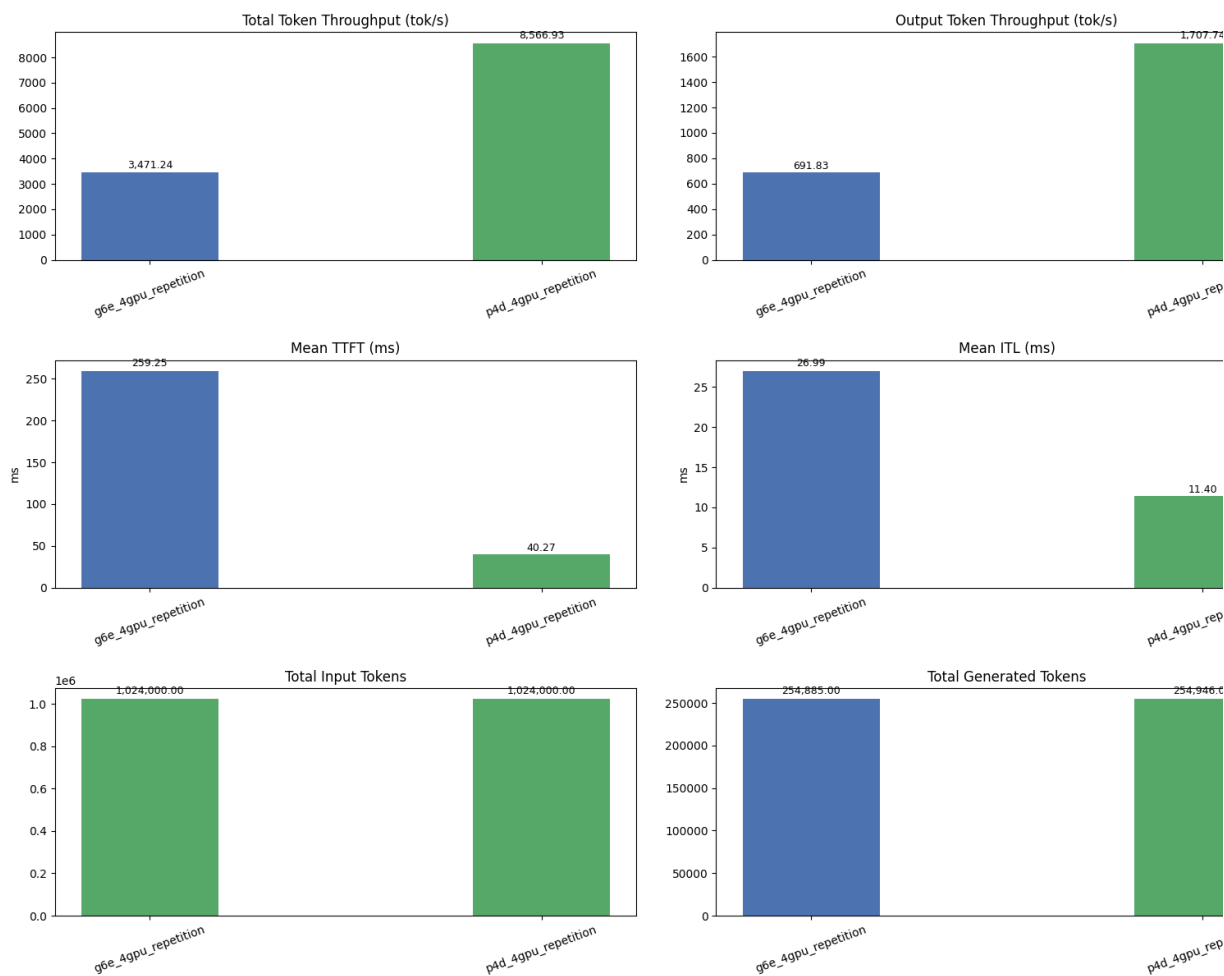
Compare NVLink performance Qwen3-14B on G6e and P4d on prefix repetition dataset
