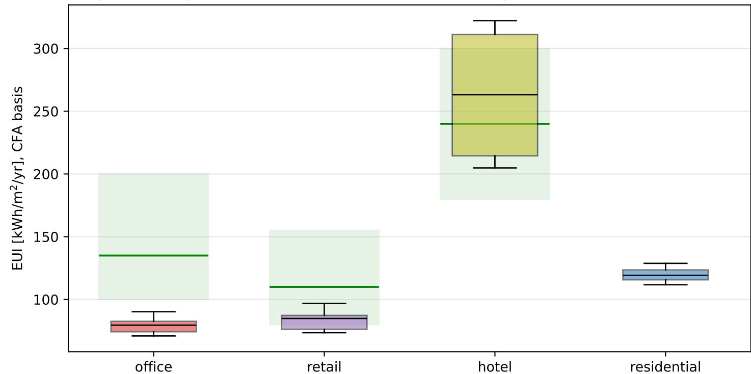
Step 9 §R1 — per-channel EUI vs as-modelled band (green) · CFA basis · all 56 cells
