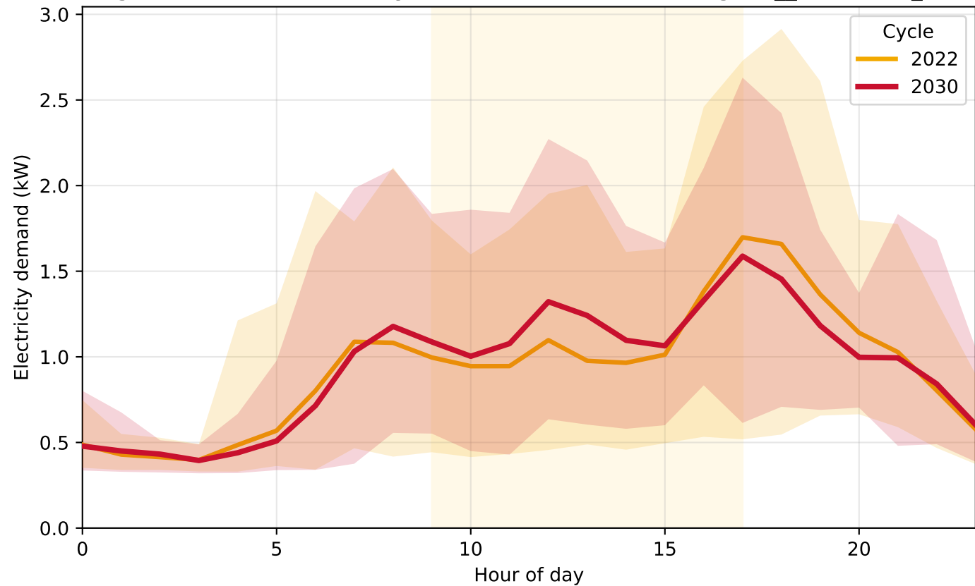
Fig 2 - Diurnal electricity load: 2022 vs 2030 (SingleD__Montreal_6A)
