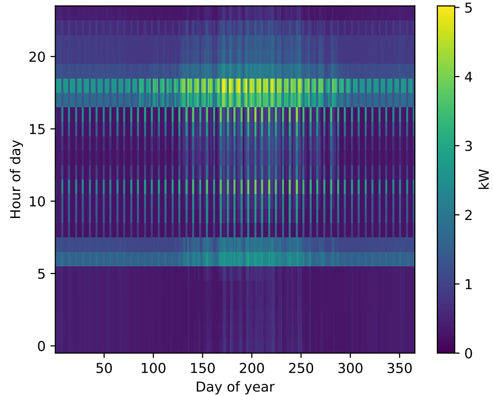
Fig 6 - Annual electricity carpet (SingleD__Montreal_6A, sample 1)
