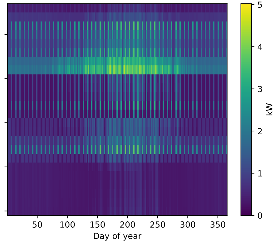
Fig 6 - Annual electricity carpet (SingleD__Montreal_6A, sample 1)
