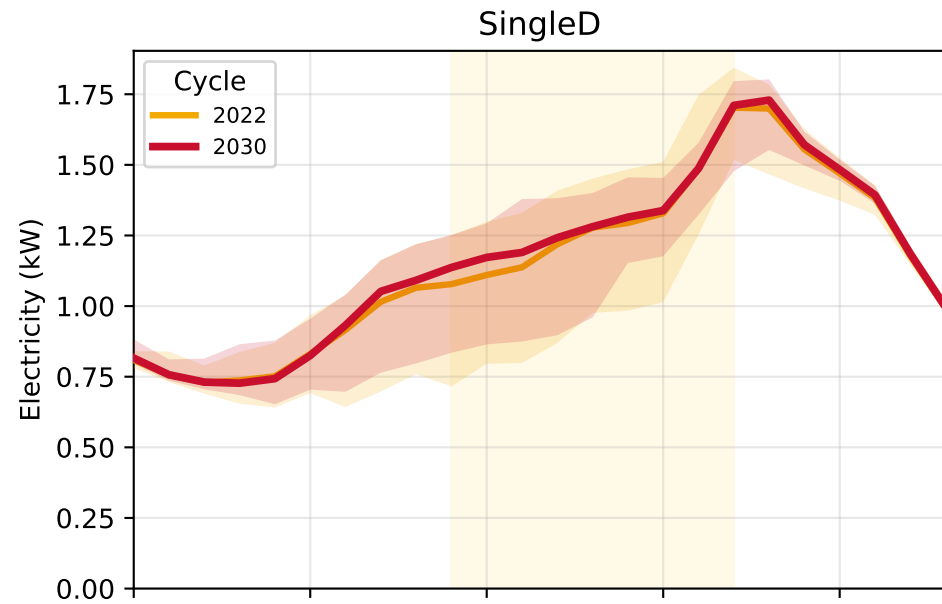
Fig 2b - Diurnal electricity by archetype (Montreal_6A)
