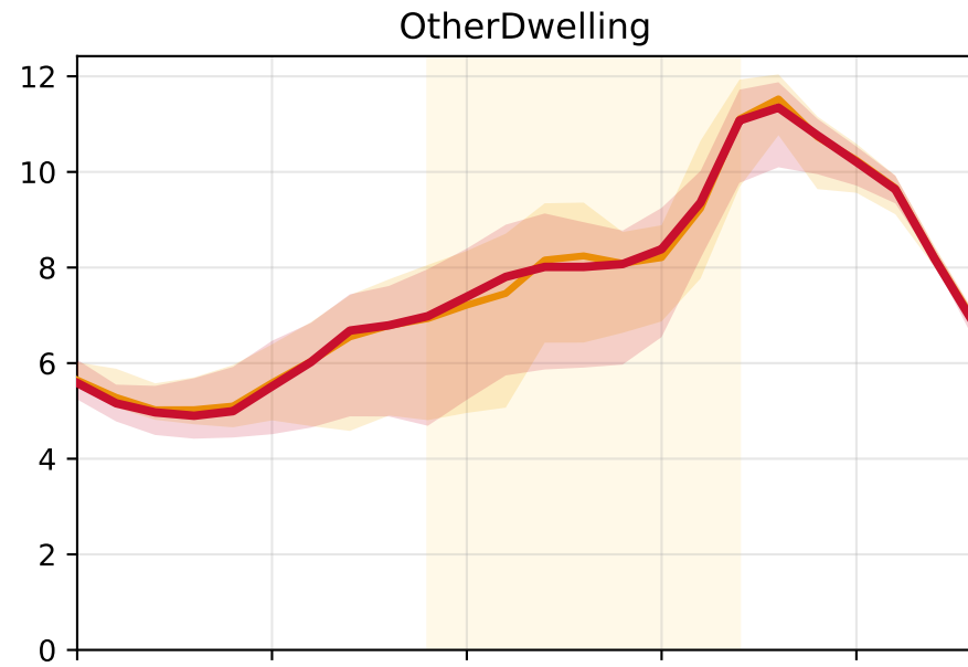
Fig 2b - Diurnal electricity by archetype (Montreal_6A)
