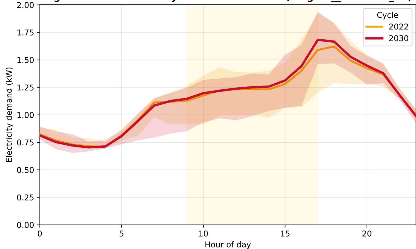
Fig 2 - Diurnal electricity load: 2022 vs 2030 (SingleD__Montreal_6A)
