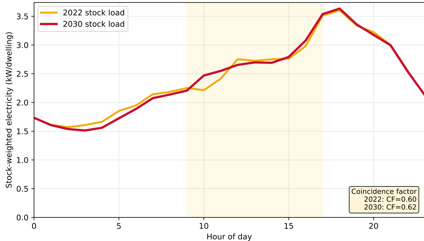
Fig 8 - Stock-weighted ensemble load shape + coincidence factor
