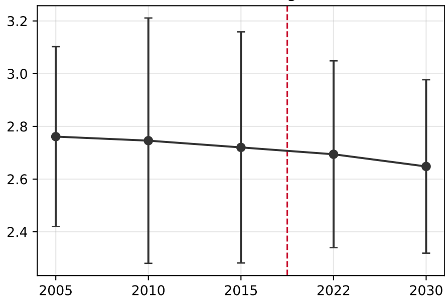
Peak-to-average
