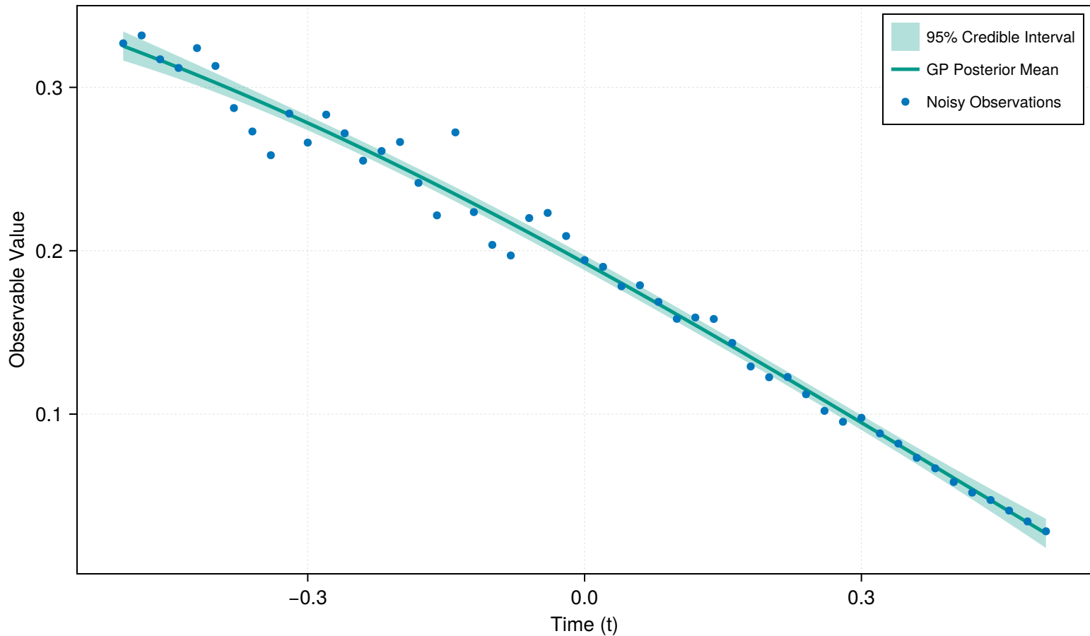
GP Interpolation with Uncertainty Bands
