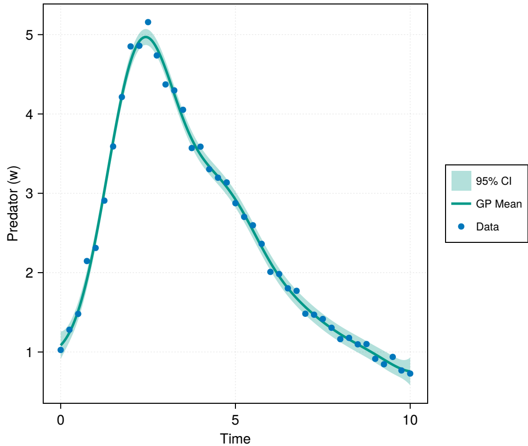
Predator Dynamics
