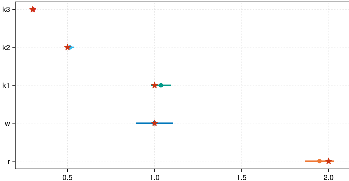
Parameter Estimates (Prey observed only)
