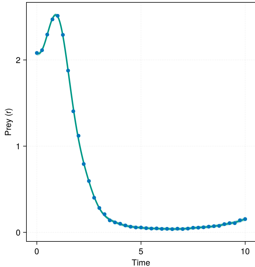
Prey Dynamics
