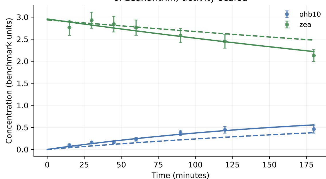
6: zeaxanthin; activity scaled
