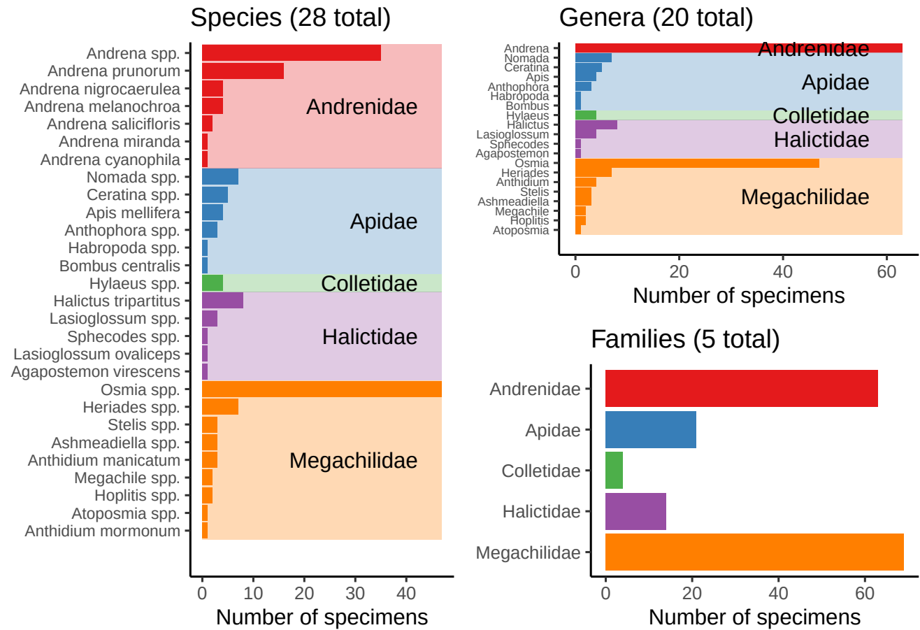
Figure 2: Bees caught by Stuart Wilson, broken down by species, genus, and family.
