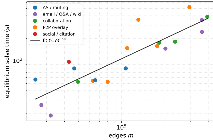
Figure 1 Equilibrium solve time vs. edge count across a topology-diverse corpus of 20 irregular SuiteSparse/SNAP graphs (seven families; peer-to-peer and collaboration largest, signed-social and messaging single instances). Wall-clock fits t \propto m^{0.90} over \approx 1.2 decades, with a bounded inner-engine setup count (in [87, 311], one build per fine \delta -level)—a descriptive near-linear trend across real graphs of every family, not a complexity estimate (Section 5).
