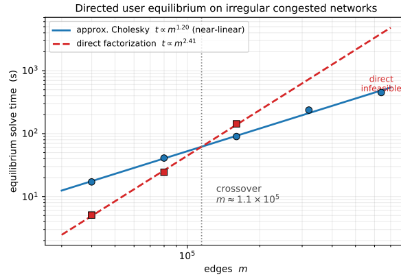
FIG. 5.1. Equilibrium solve time vs. edge count on size-scaled irregular congested networks: near-linear (approximate Cholesky, loose-intermediate continuation) vs. superlinear (direct factorization), crossing near m \approx SCROSS .
