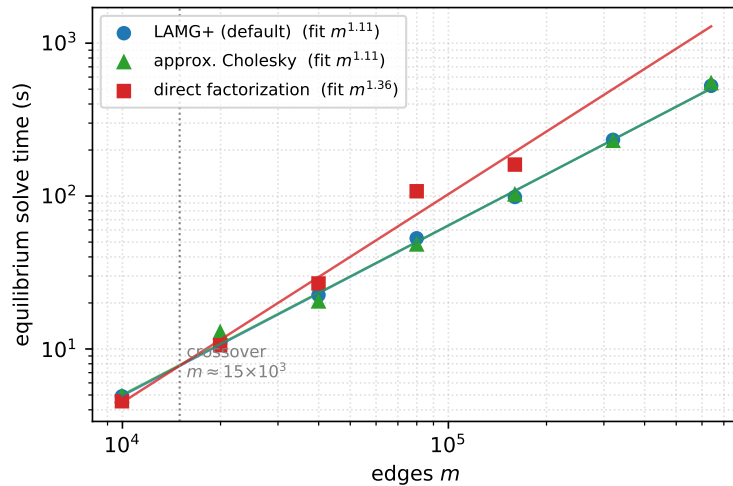
Figure 2 Equilibrium solve time vs. edge count on size-scaled irregular congested networks: the two near-linear engines—LAMG+ (default) and approximate Cholesky, both fitting m^{1.11} —vs. superlinear direct factorization ( m^{1.36} ), the near-linear engines crossing the direct baseline near m \approx 1.5 \times 10^4 .
