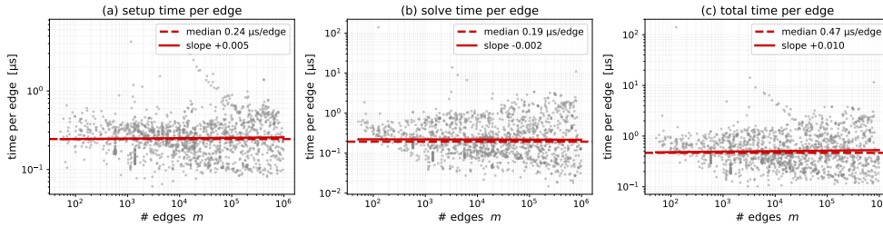
LAMG+ linear scaling — 1,711 real-world graph Laplacians ( m = 52..982,542 )
