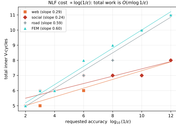
FIG. 4.4. Cost vs. desired accuracy: total inner V-cycles against \log_{10}(1/\epsilon) , one graph per class. The count is linear in \log(1/\epsilon) (0.24–0.60 cycles per decade), confirming the total cost \mathcal{O}(m \log(1/\epsilon)) of (4.2).
