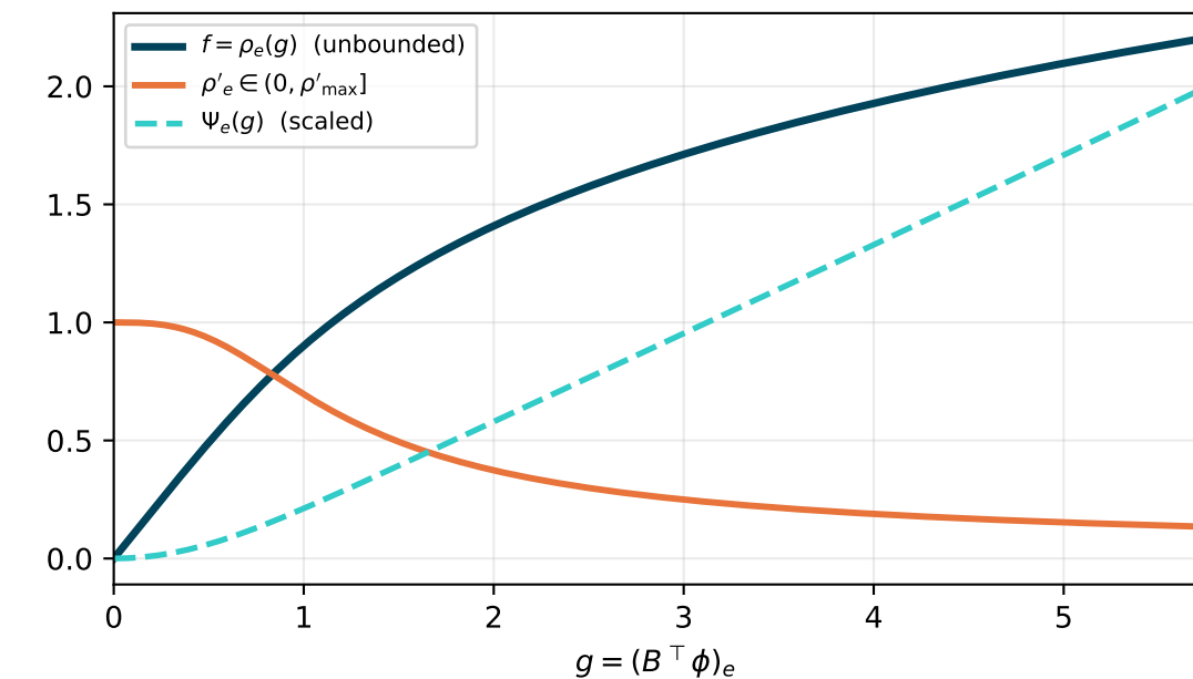
(A3) congestion (BPR): no cap, conductance bounded \Rightarrow no fold
