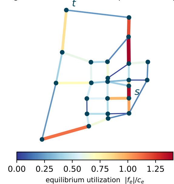
(B3) congestion: Sioux Falls, computed NLF equilibrium
