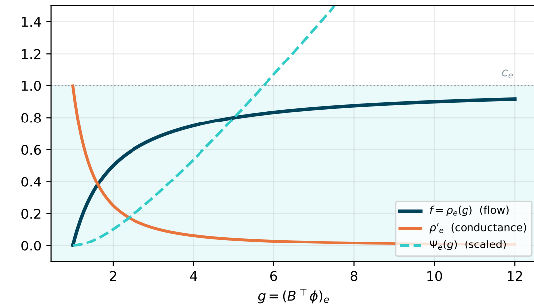
(A2) min-delay (Kleinrock 1/(c_e - f) ): saturates at capacity
