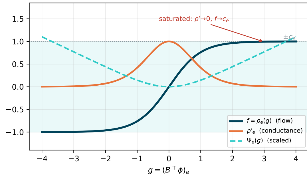
(A1) max-flow: saturating law, \rho' \rightarrow 0 at the cut
