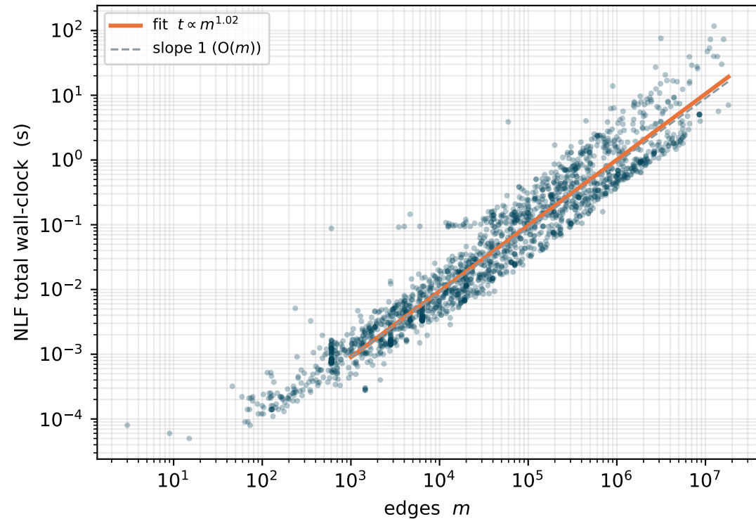
(A) t \propto m^{1.02} over 1788 real graphs: genuine O(m)
