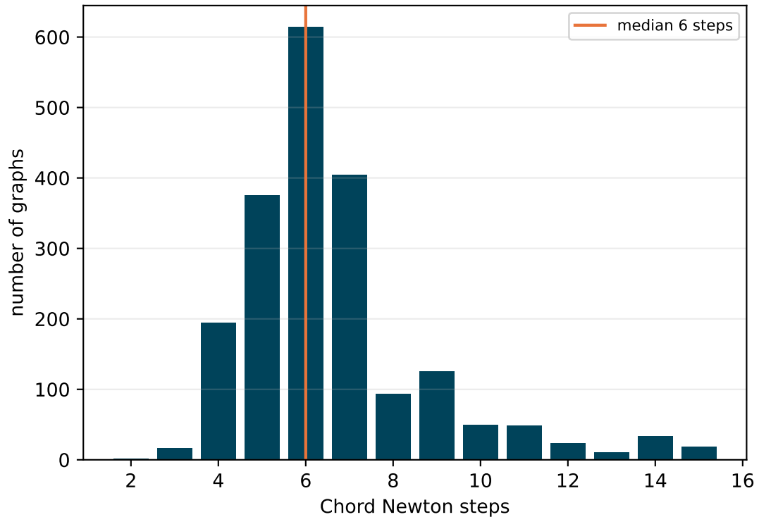
(B) chord-Newton step count: flat in size and class
