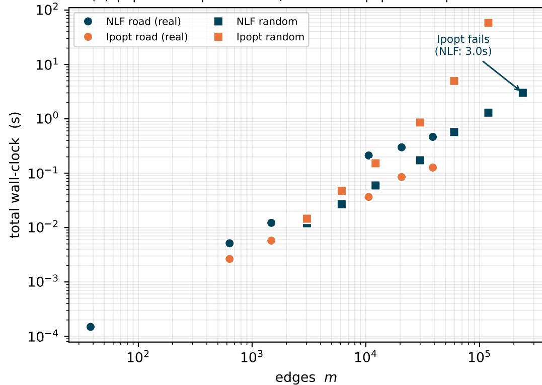
(B) Ipopt wins on planar roads; NLF wins + Ipopt blows up on random
