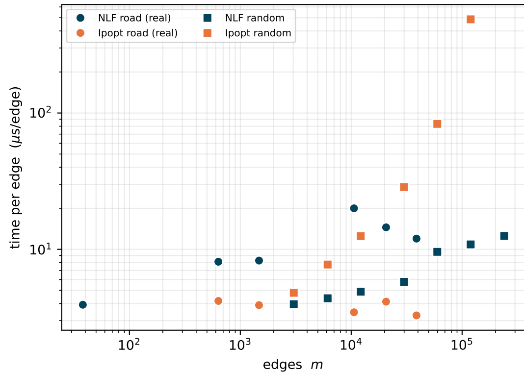
(A) Per-edge: NLF flat ( O(m) ) vs Ipopt rising on random ( \propto m^{1.19} )
