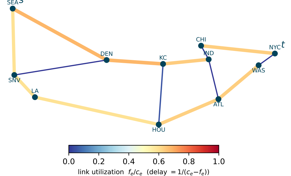
(B2) min-delay: Abilene backbone, computed FAMG equilibrium
