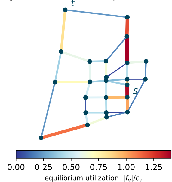
(B3) congestion: Sioux Falls, computed FAMG equilibrium
