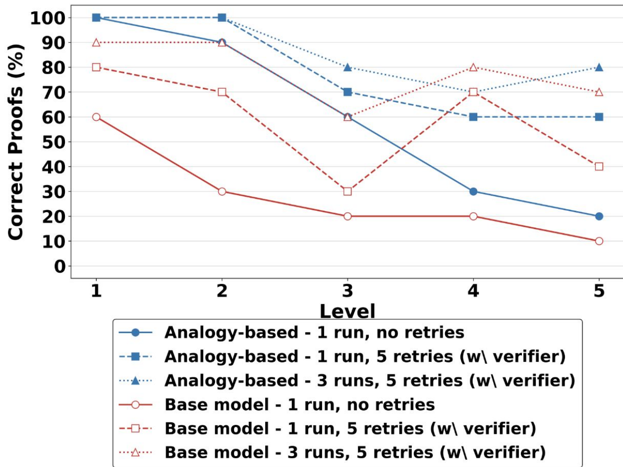
% correct proofs per level of difficulty
