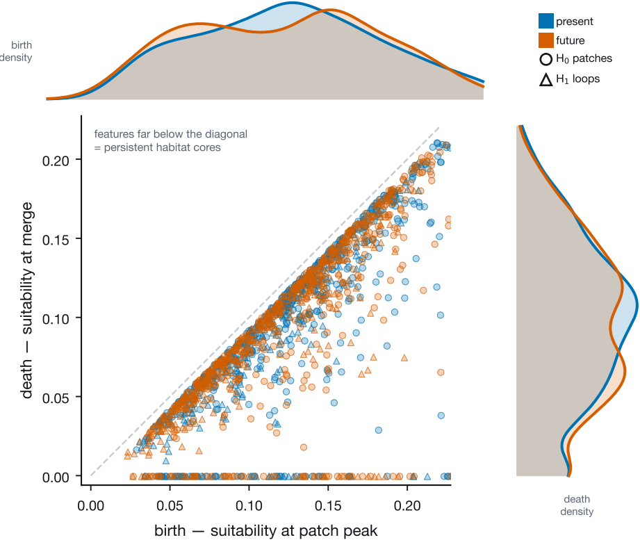
c Persistence diagram: shape of the range
