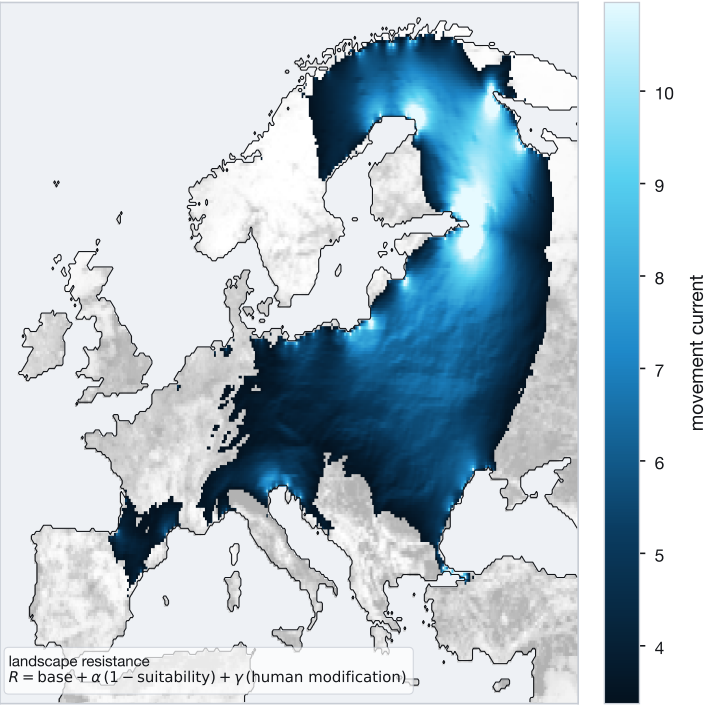
a Climate-forced movement routed through landscape
