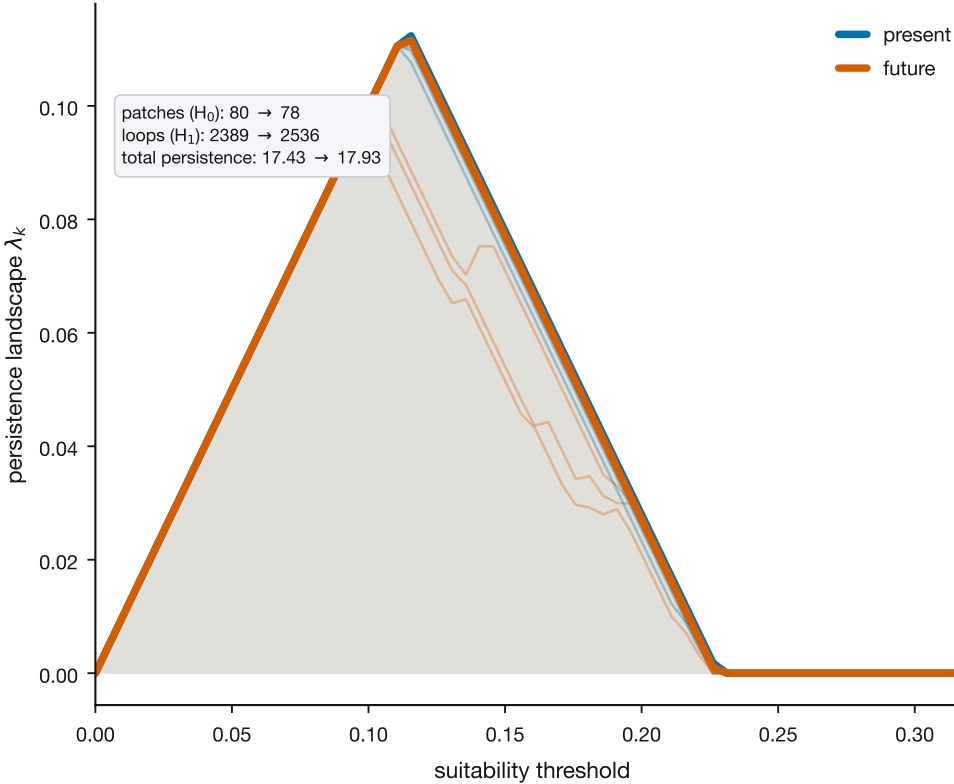
d Topological simplification of habitat
