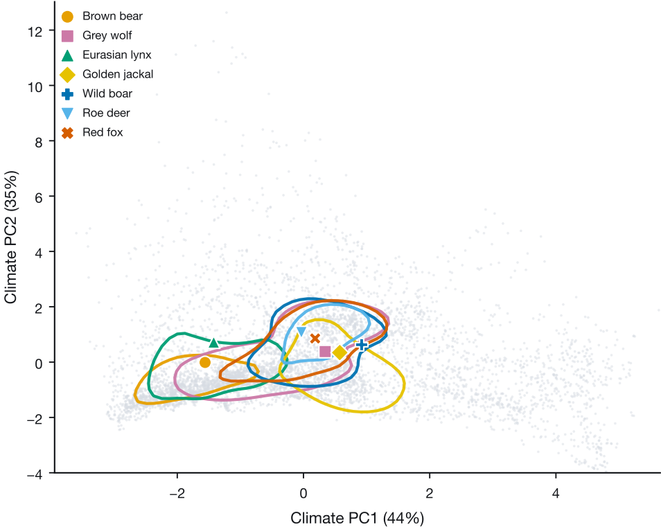
b Realized climatic niches (bioclim PCA)
