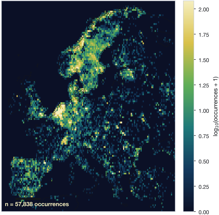
a Georeferenced records across 7 conflict-prone taxa
