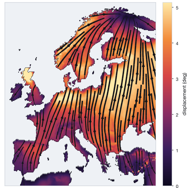
b Entropic displacement field T(x) - x
