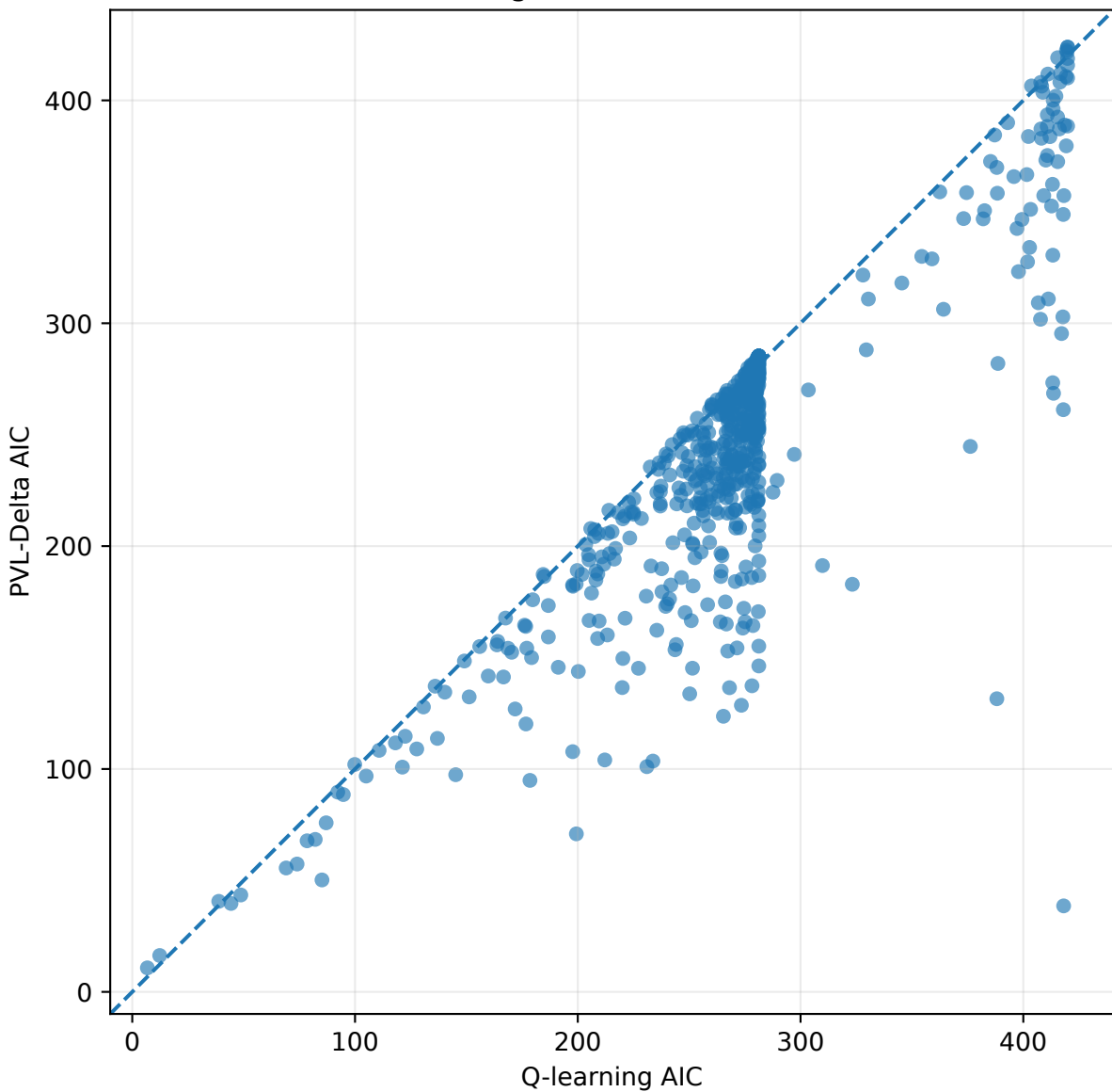
Q-learning versus PVL-Delta AIC
