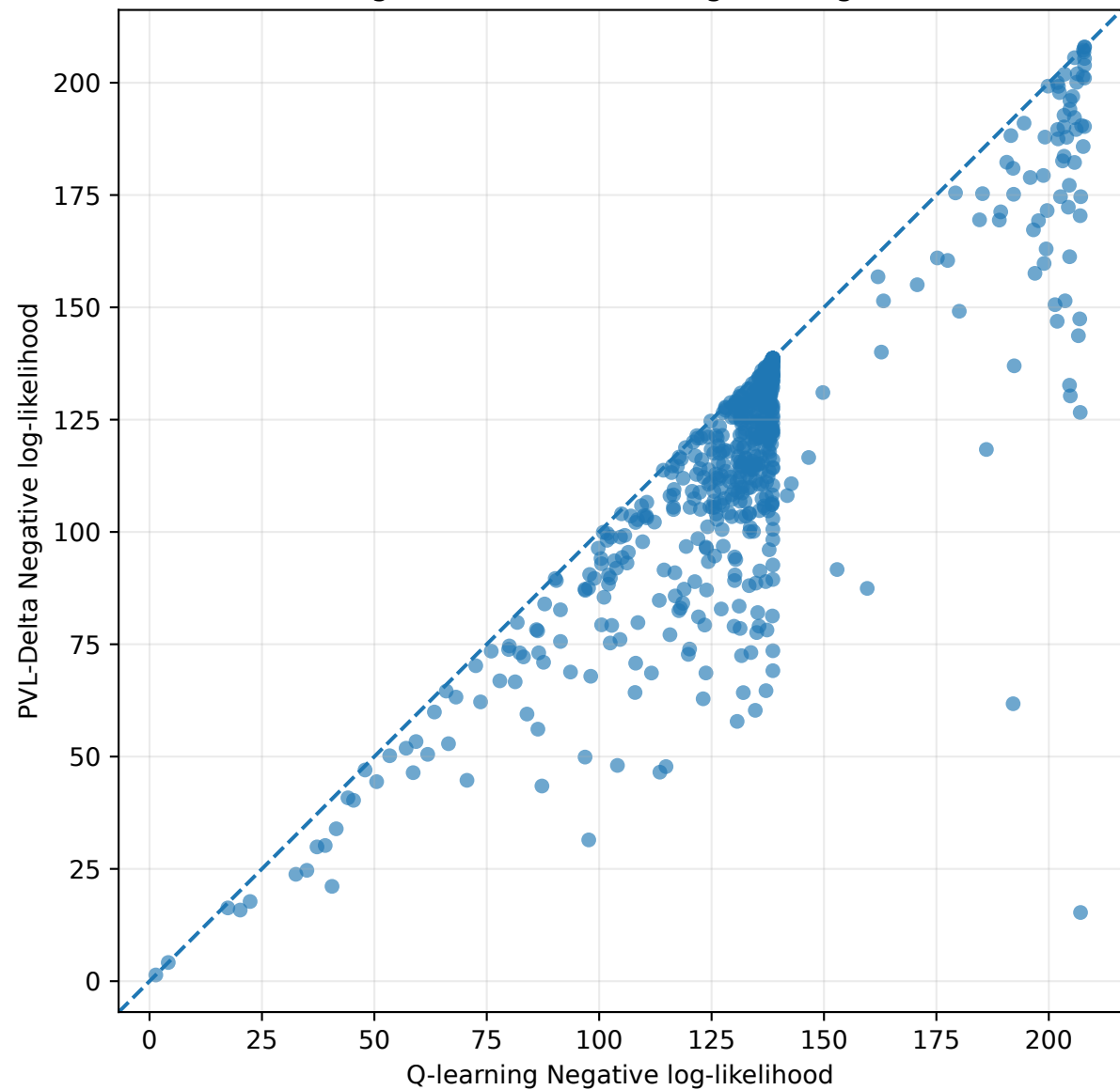
Q-learning versus PVL-Delta Negative log-likelihood
