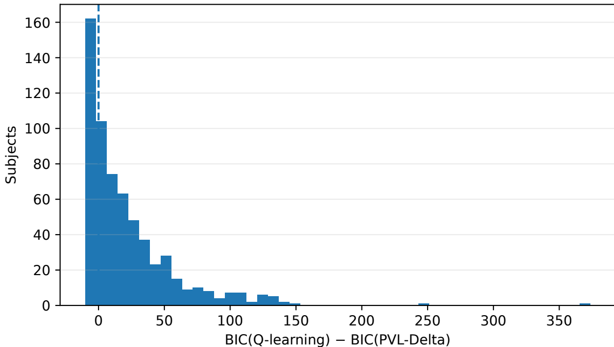
Distribution of signed BIC differences
