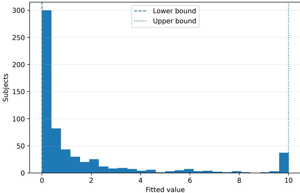
PVL-Delta: loss aversion ( \lambda )
