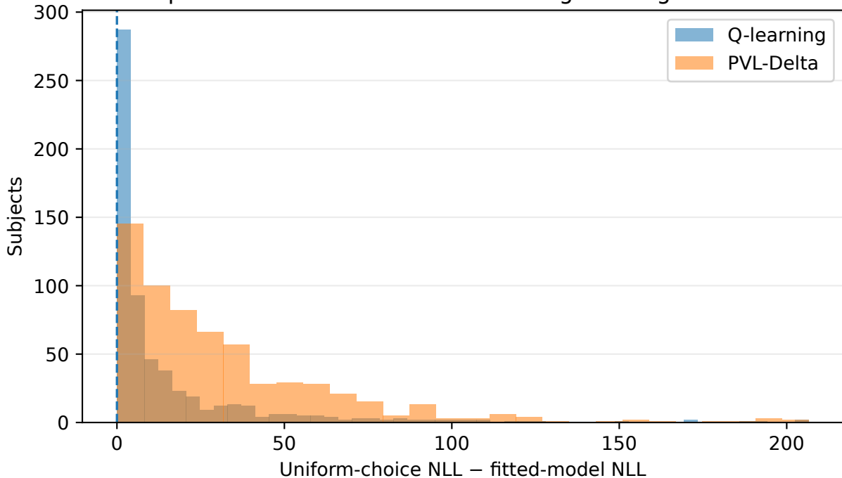
Improvement over uniform-choice negative log-likelihood
