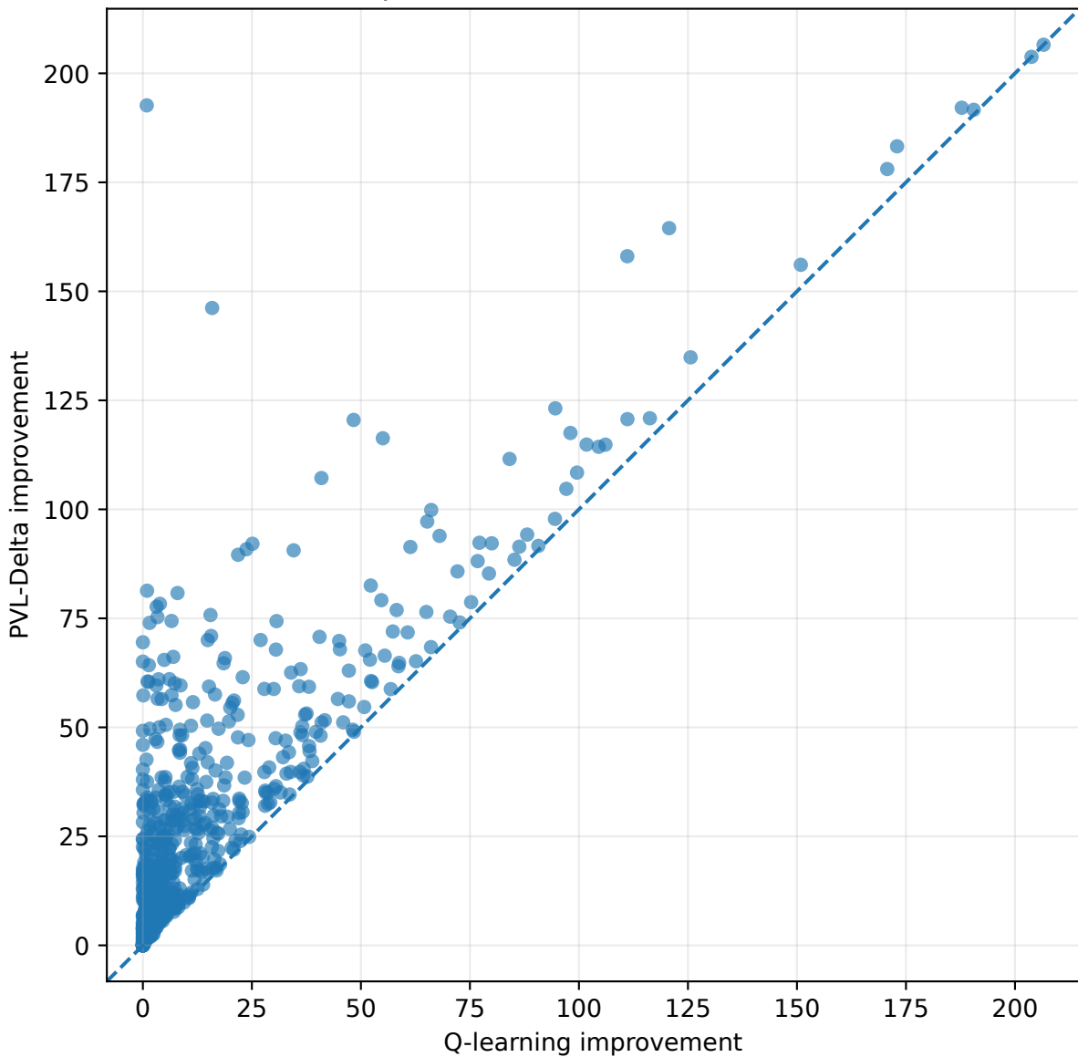
Improvement over uniform choice
