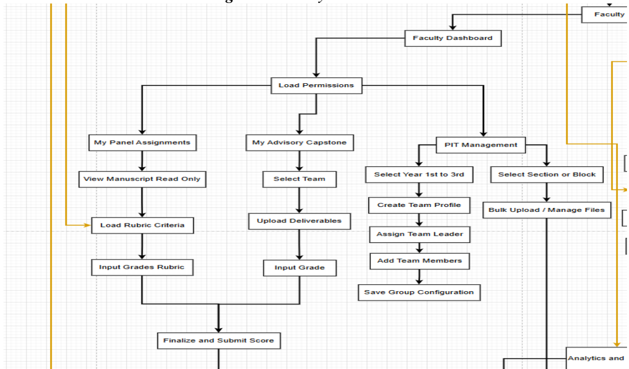
Figure 5: Faculty Side
