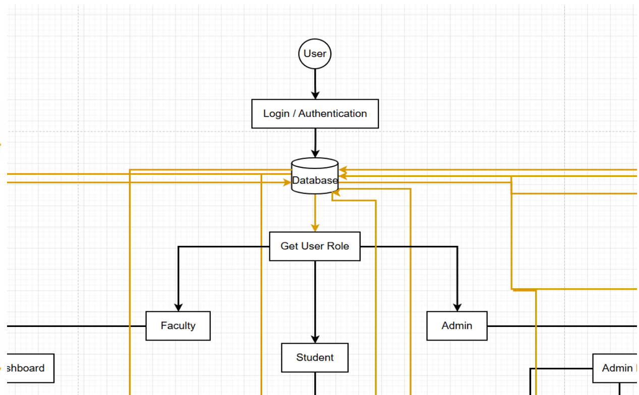
Figure 2: Login Process
