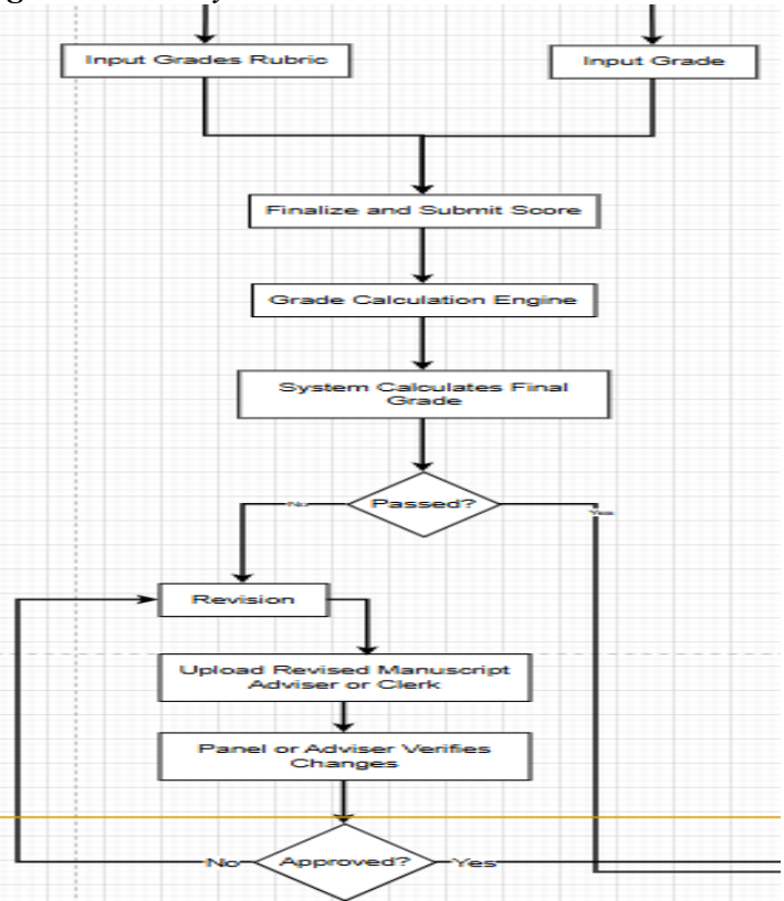
Figure 6: Faculty Side
