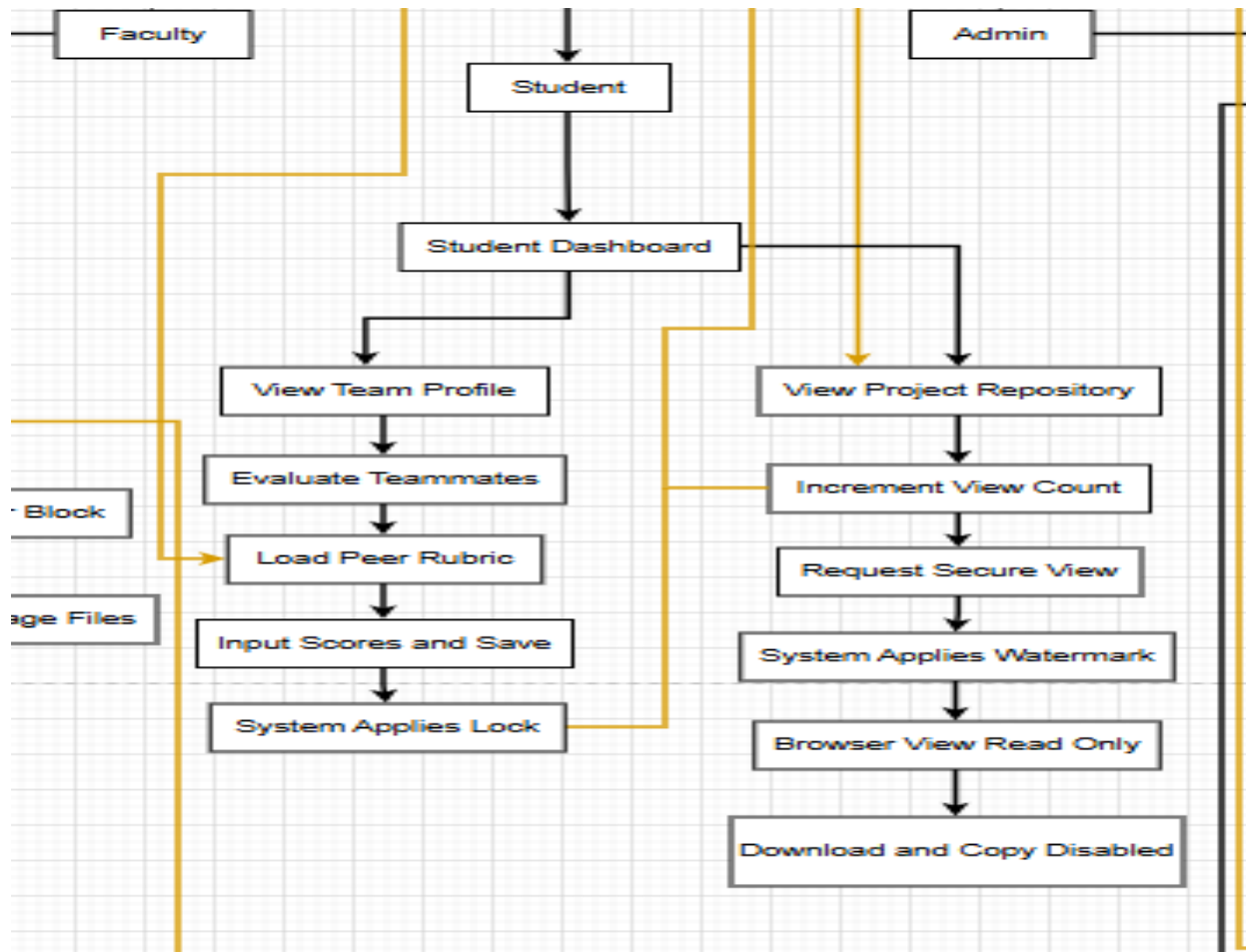
Figure 7: Student Side
