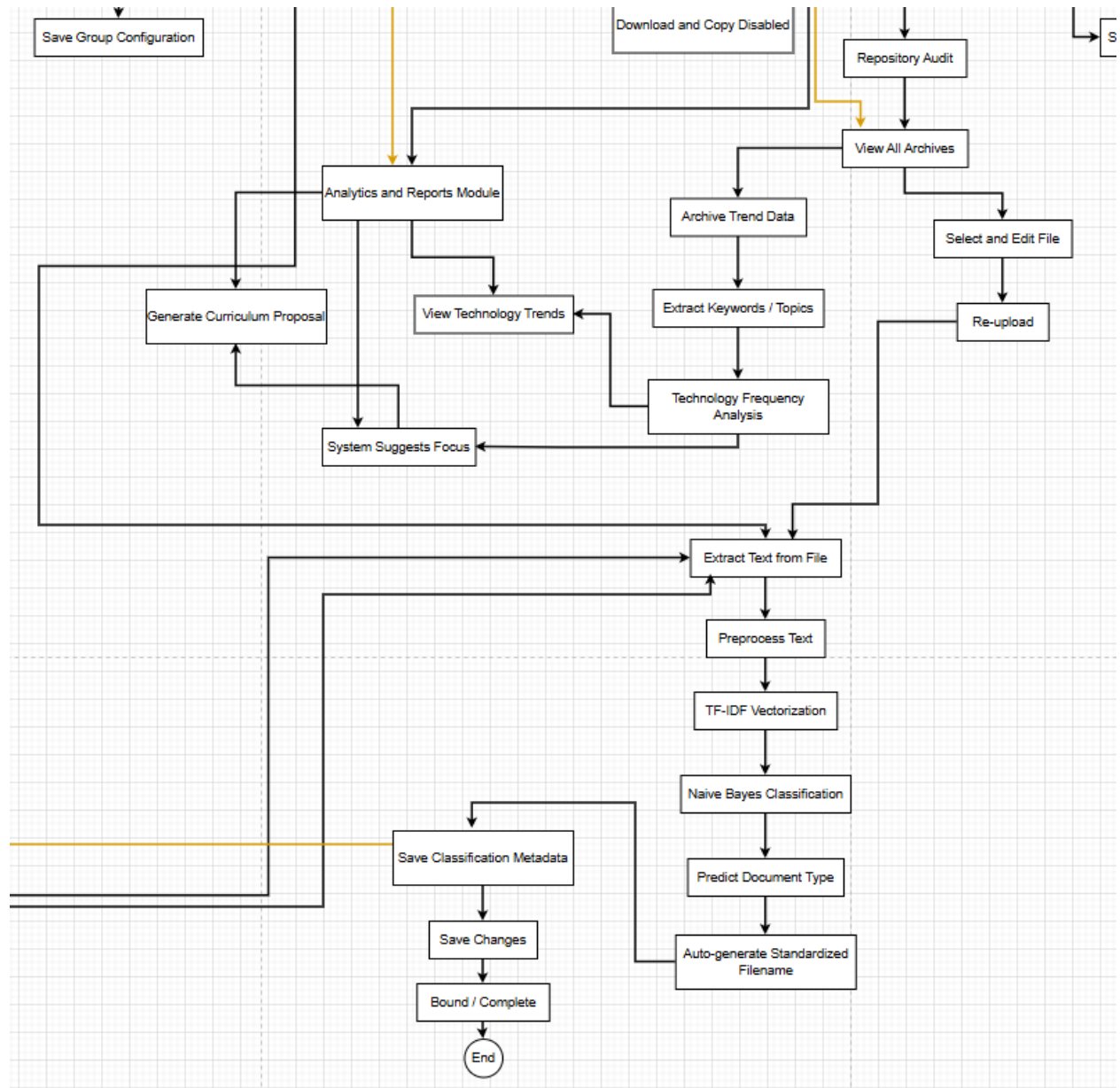
Figure 4: Admin Side
