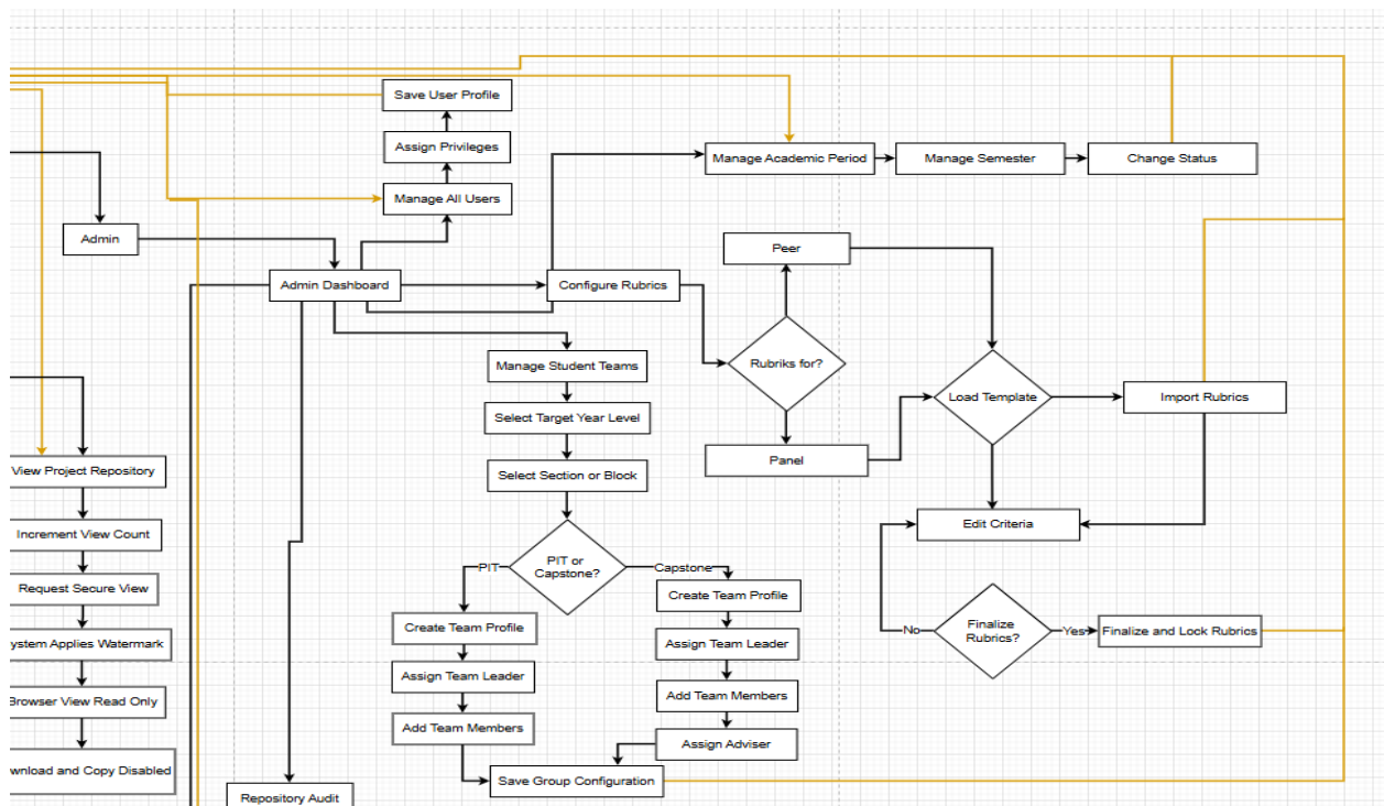
Figure 3: Admin Side
